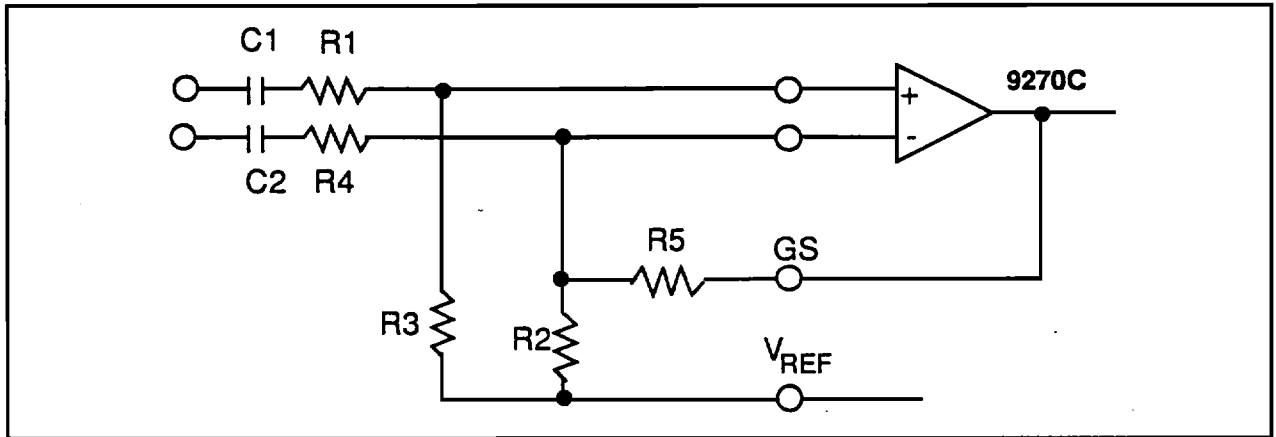
FIGURE 8. DIFFERENTIAL INPUT CONFIGURATION
