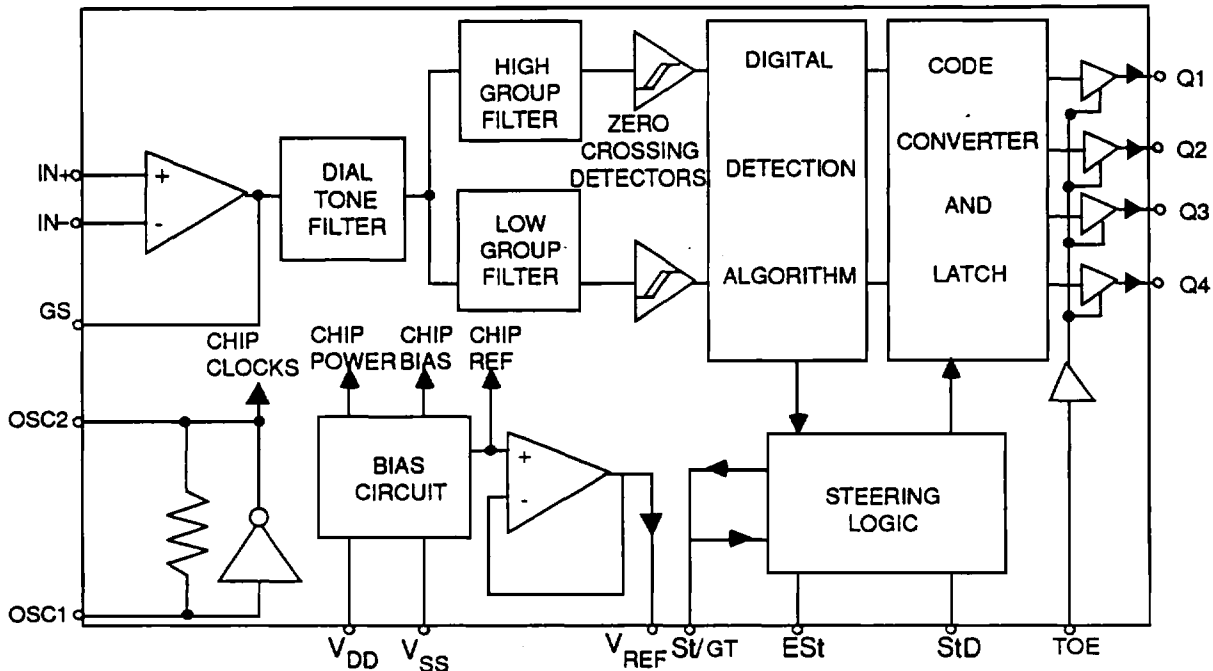
Block Diagram (Figure 1)
