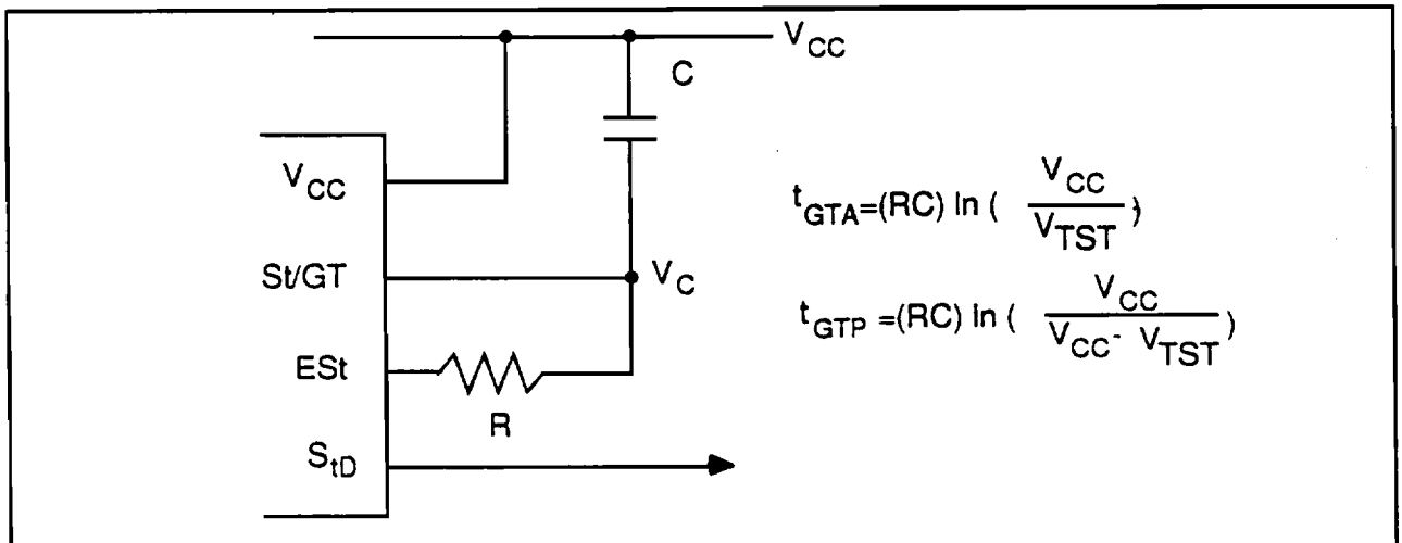
FIGURE 6. BASIC STEERING CIRCUIT
