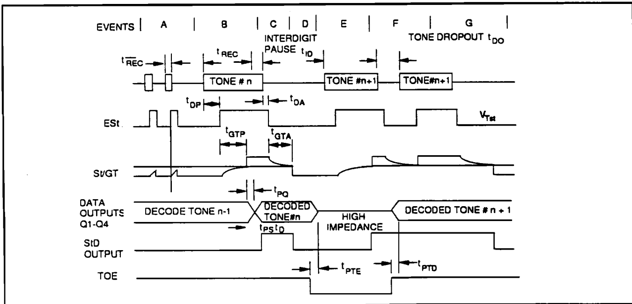
FIGURE 4. TIMING DIAGRAM
