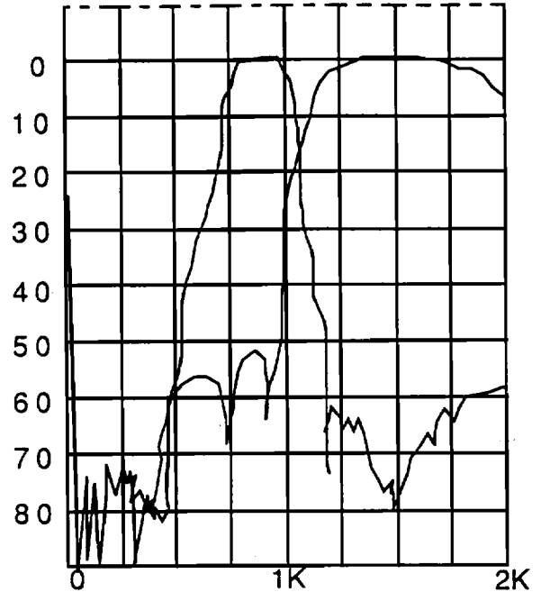
FIGURE 5. TYPICAL FILTER CHARACTERISTIC
