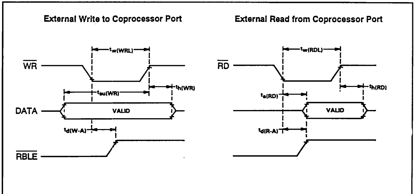
Figure 9 Coprocessor Timing
