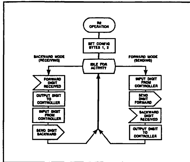
Figure 2 Automatic Compelled Mode Operation
