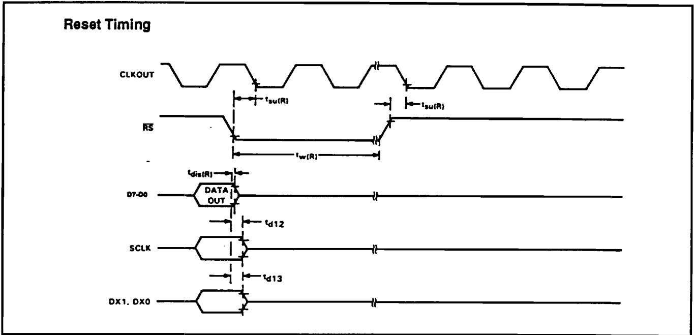
Figure 8 Reset Timing
