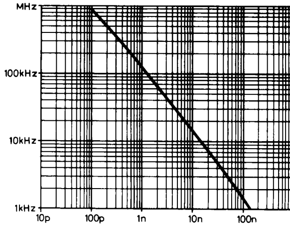
Fig. 8 Typical clock frequency v C_{CK} ( R_{CK} = 0 )
