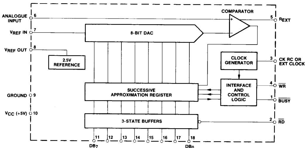
Fig.1 System diagram
