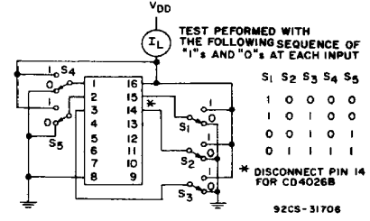
Fig. 15 - Quiescent device current.
