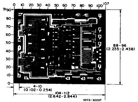
Dimensions and pad layout for CD4033B.
