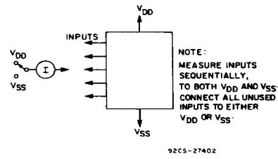
Fig. 17 - Input current.
