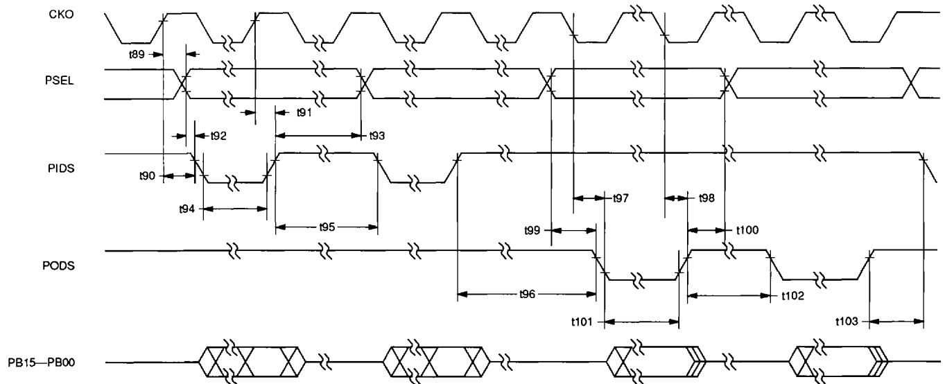
Figure 13. Parallel I/O Active Timing
