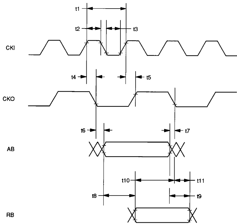
Figure 4. External Memory Interface
