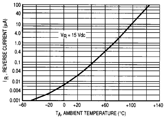
Figure 4. Leakage Current
