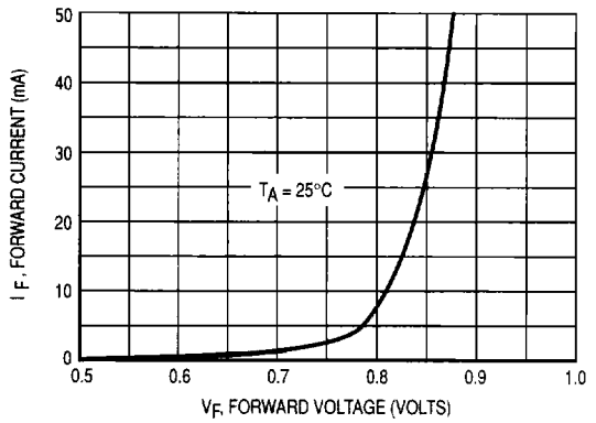
Figure 2. Forward Voltage
