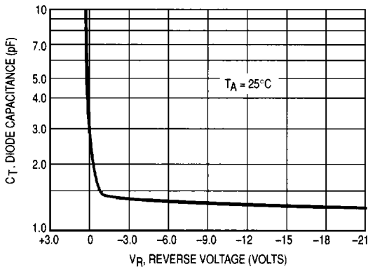
Figure 3. Diode Capacitance
