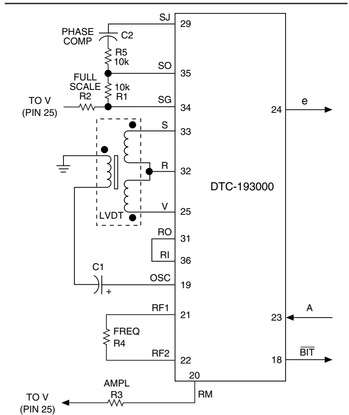
FIGURE 7. DTC-19300 SET-UP
