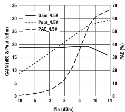
Figure 34. Small Signal Gain/Pout/PAE vs. Pin at V_{ds} = 4.5V and Frequency = 900 MHz.
