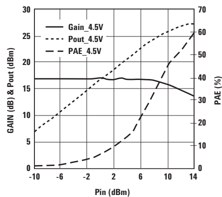
Figure 15. Small Signal Gain/Pout/PAE vs. P_{in} at V_{ds} = 4.5V and Frequency = 900 MHz.
