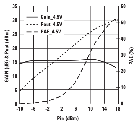
Figure 37. Small Signal Gain/Pout/PAE vs. Pin at V_{ds} = 4.5V and Frequency = 2 GHz.
