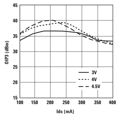
Figure 9. OIP3 vs. I_{ds} and V_{ds} at 3.9 GHz.
