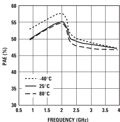
Figure 25. PAE vs. Temperature and Frequency at optimum OIP3.
