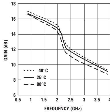
Figure 42. Gain vs. Temperature and Frequency at optimum P1dB.
