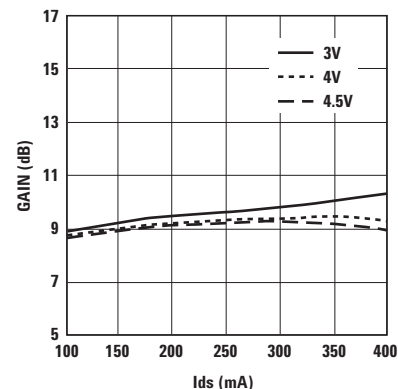
Figure 31. Small Signal Gain vs. I_{ds} and V_{ds} at 3.9 GHz.
