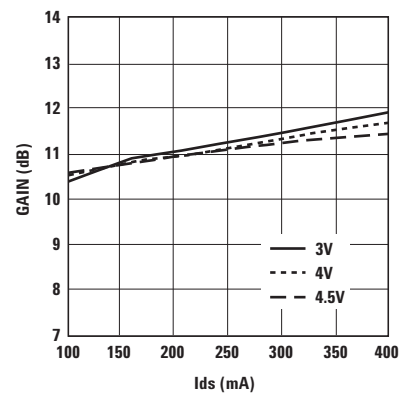
Figure 12. Small Signal Gain vs. I_{ds} and V_{ds} at 3.9 GHz.
