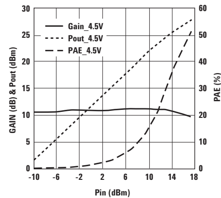
Figure 21. Small Signal Gain/Pout/PAE vs. Pin at V_{ds} = 4.5V and Frequency = 3.9 GHz.
