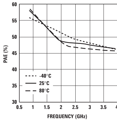
Figure 44. PAE vs. Temperature and Frequency at optimum P1dB.
