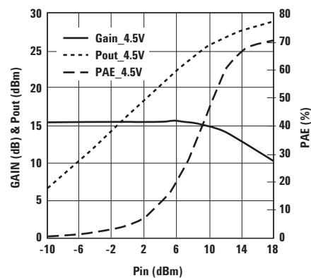
Figure 18. Small Signal Gain/Pout/PAE vs. Pin at V_{ds} = 4.5V and Frequency = 2 GHz.
