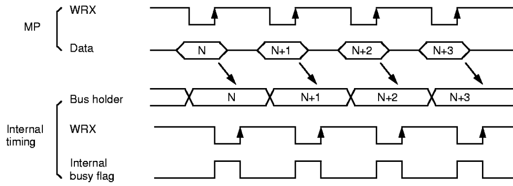
Figure 4 Display data write timing (80 family interface)
