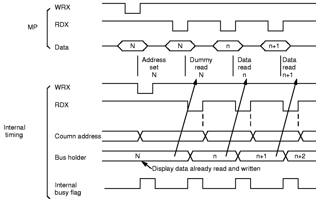
Figure 5 Display data read timing (80 family interface)
