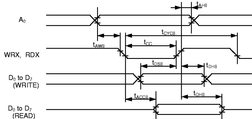
Figure 2 Read/write timing with 80 family MPU
