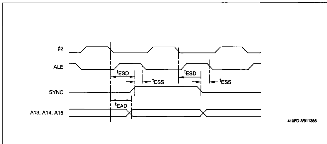
Expansion Bus Waveforms - R65C19 Emulator
