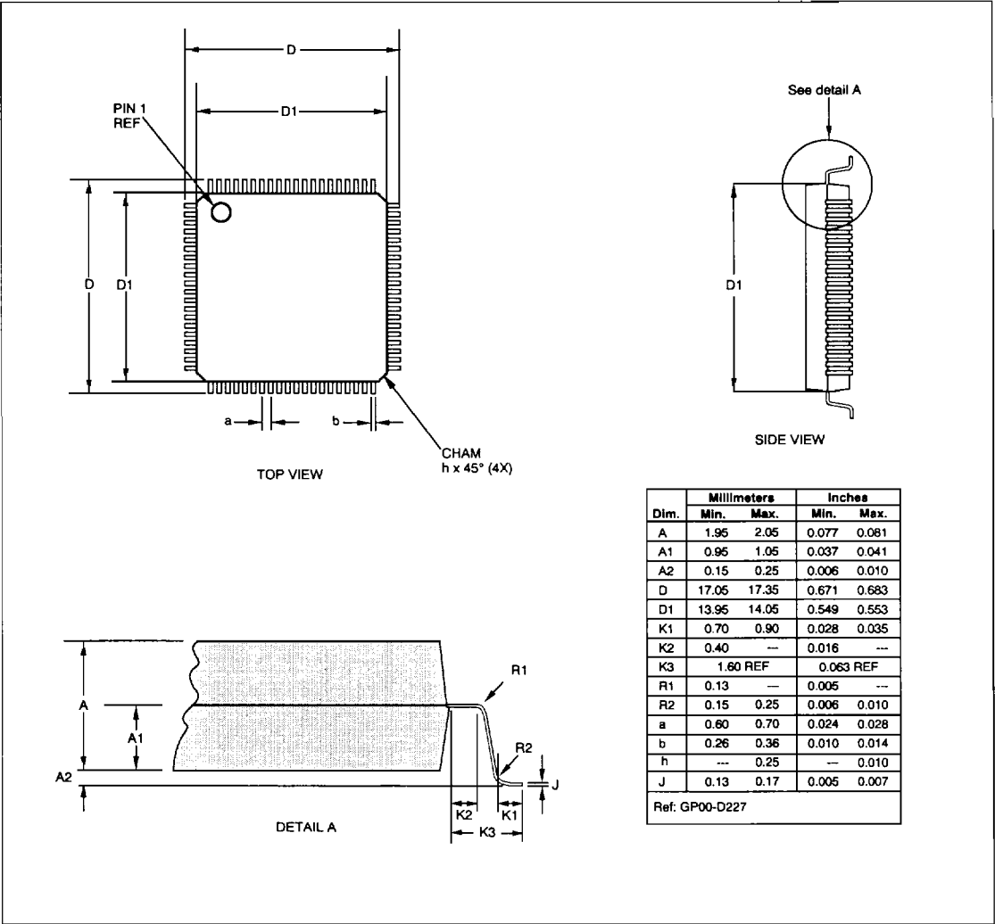
80-Pin PQFP
