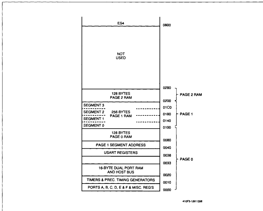
Figure 3-1. RAM Register Memory Map
