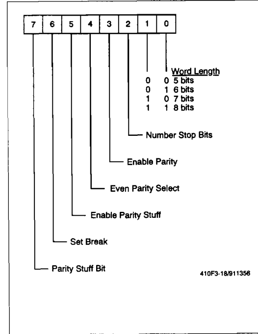
Figure 3-18. Serial Line Register (SLR) - $003B
