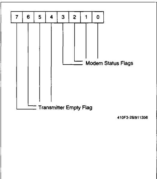
Figure 3-28. Modem Status Register (MSR) - $0031
