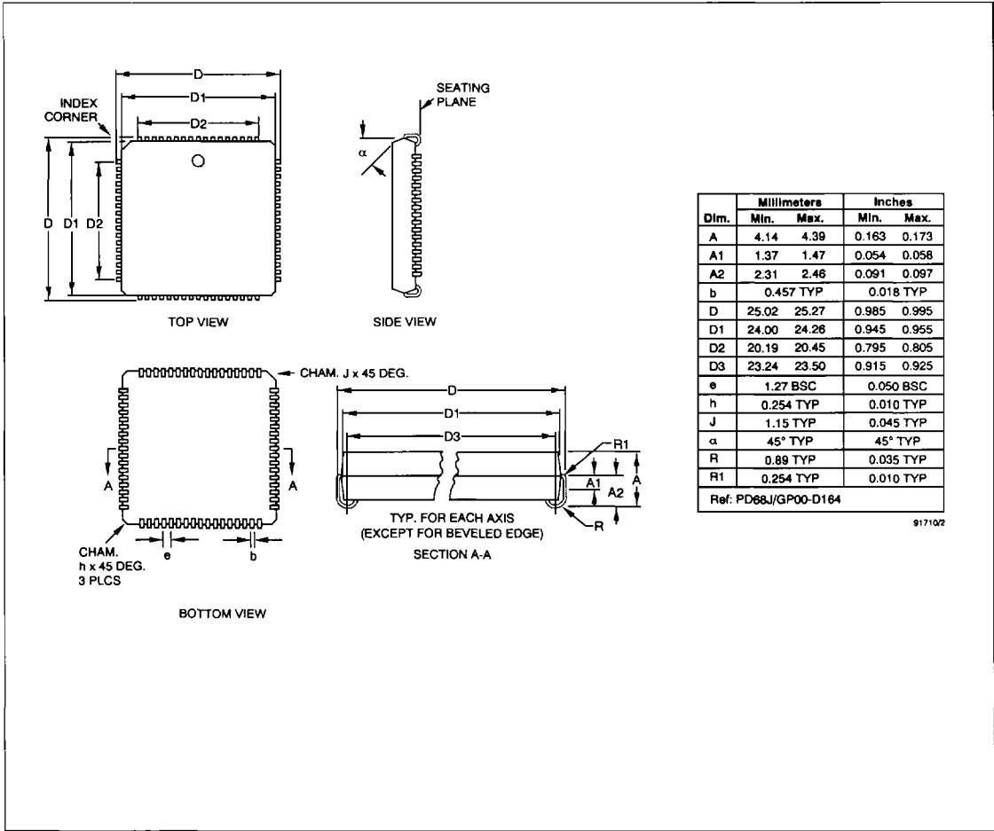
68-Pin PLCC
