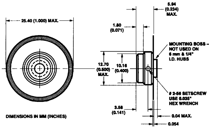
Figure 4. HEDS-5120 Codewheel.
