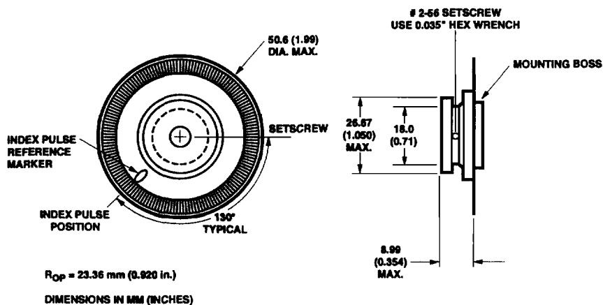
Figure 7. HEDS-6140 Codewheel Used with HEDS-9040.
