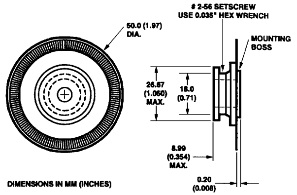
Figure 5. HEDS-6100 Codewheel.
