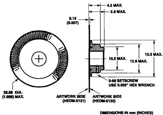
Figure 8. HEDM-5120 Codewheel/HEDM-5121 Codewheel.
