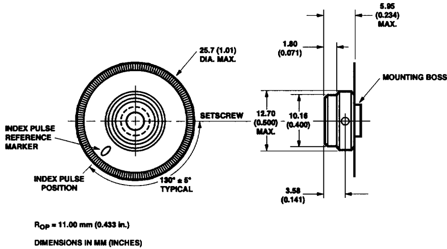
Figure 6. HEDS-5140 Codewheel Used with HEDS-9140.
