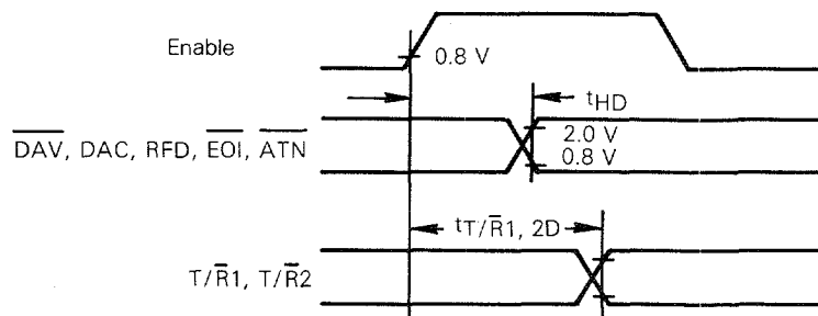
FIGURE 5 — OUTPUT BUS TIMING
