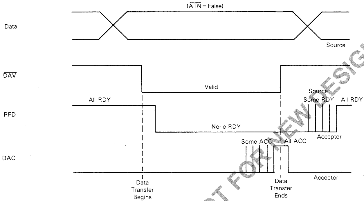
FIGURE 3 — SOURCE AND ACCEPTOR HANDSHAKE
