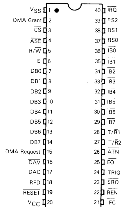
FIGURE 1 — PIN ASSIGNMENT
