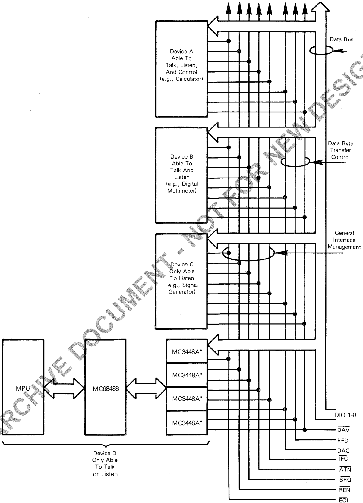
FIGURE 7 — GPIB SYSTEM
