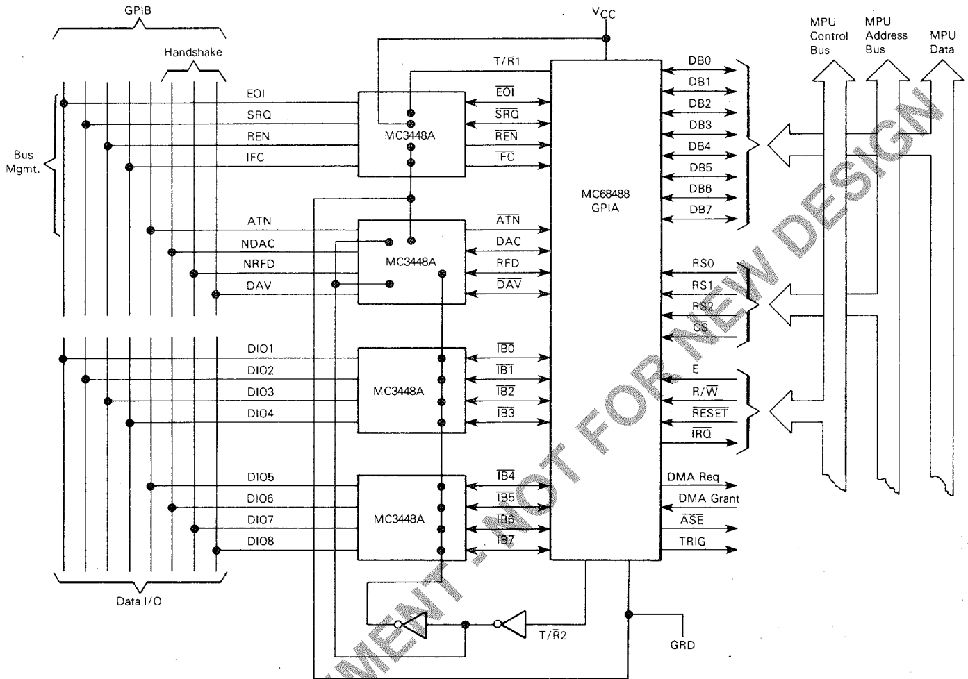
FIGURE 2 — GPIB INTERFACE
