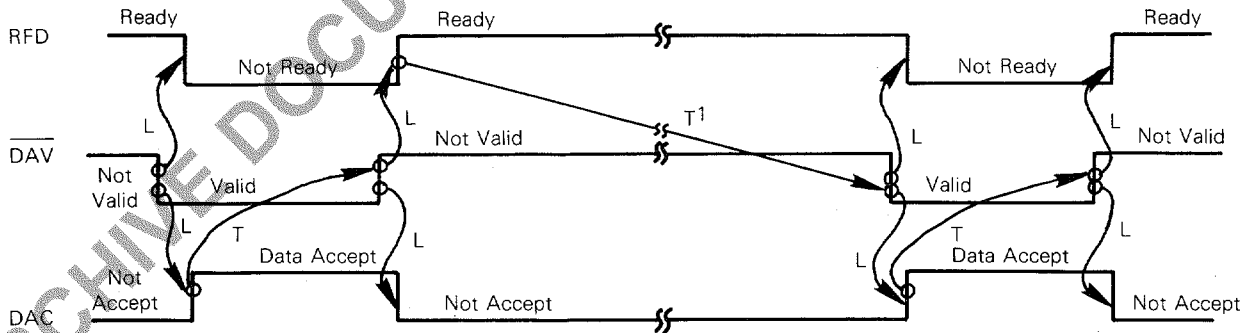
FIGURE 9 — GPIA IN TALKER MODE*
