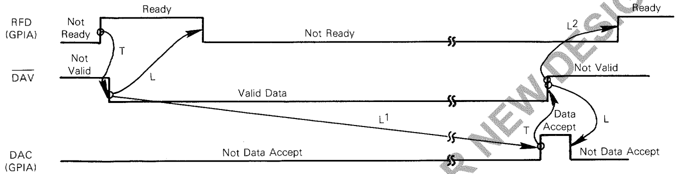
FIGURE 8 — GPIA IN LISTEN MODE*
