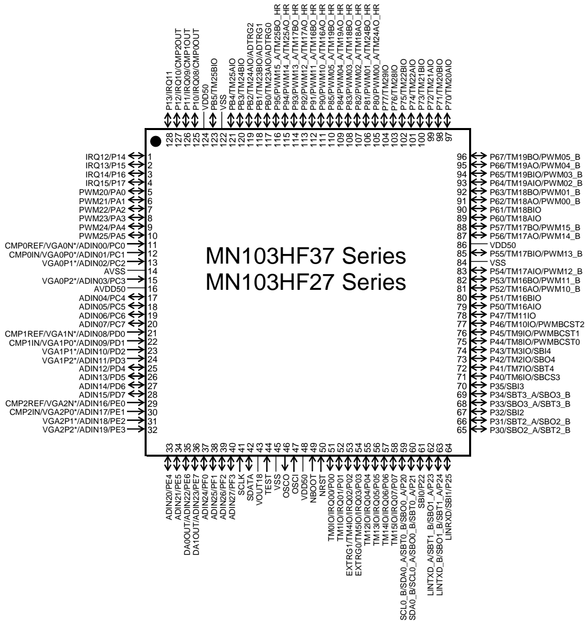
Figure:1.4.2 Pin Configuration of MN103HF37/27 Series
