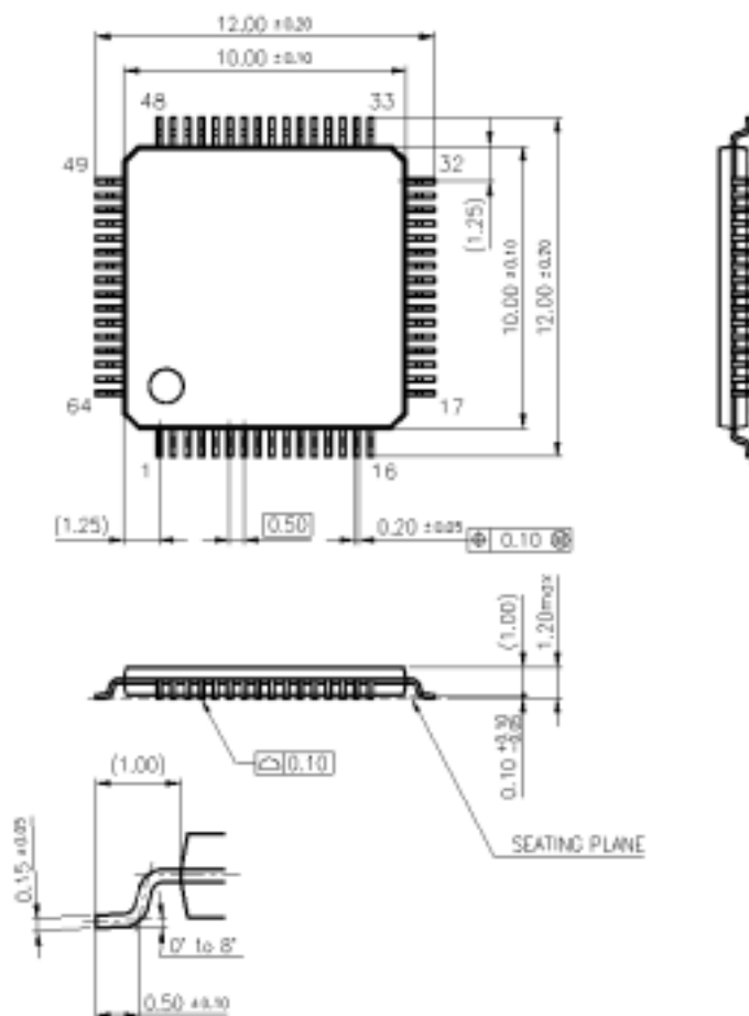
Figure:1.7.6 Package Dimension of 64 pin TQFP
