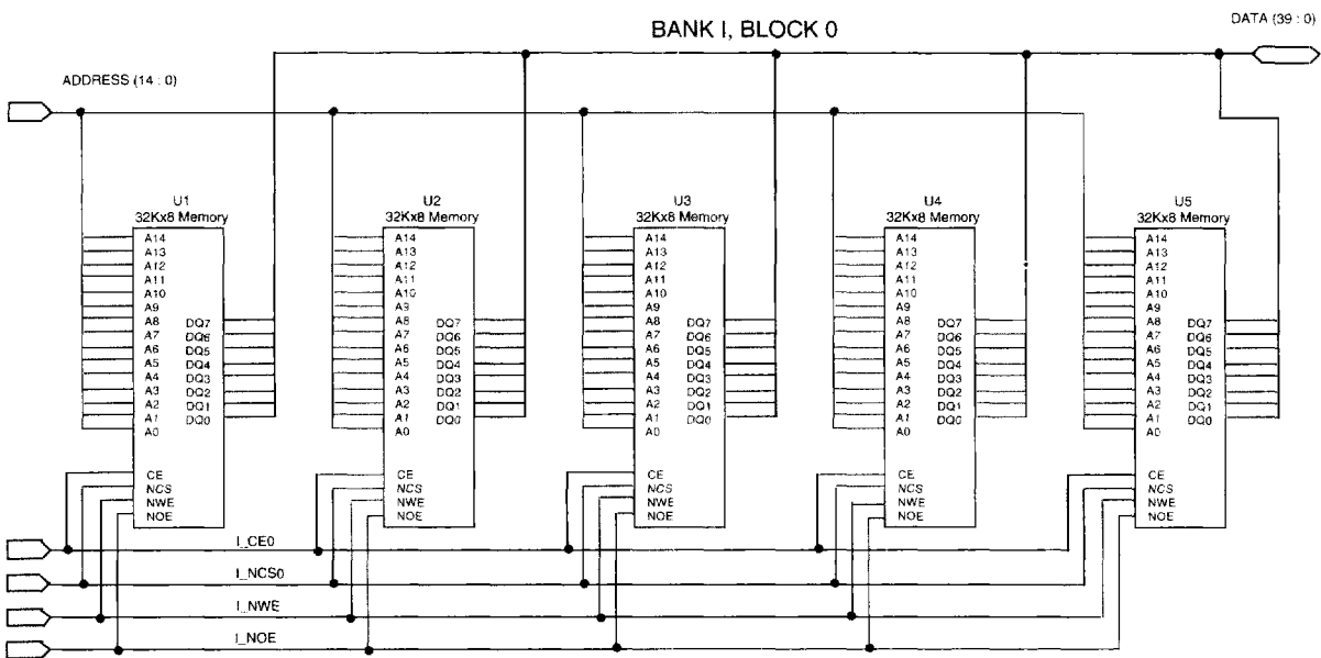
Figure 2. 32K x 40 Memory Block Functional Diagram
