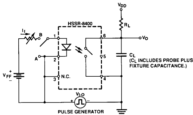
Figure 16. Output Transient Rejection Test Circuit.
