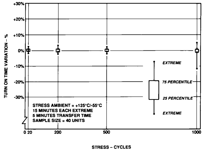
Figure 21. Turn On Time Variation with Temperature Cycling.
