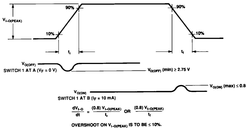
Figure 17. Input-Output Transient Rejection Test Circuit.
