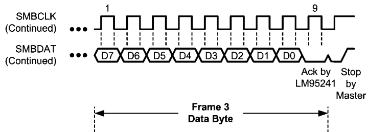
(b) Serial Bus Write to the internal Command Register followed by a Data Byte
