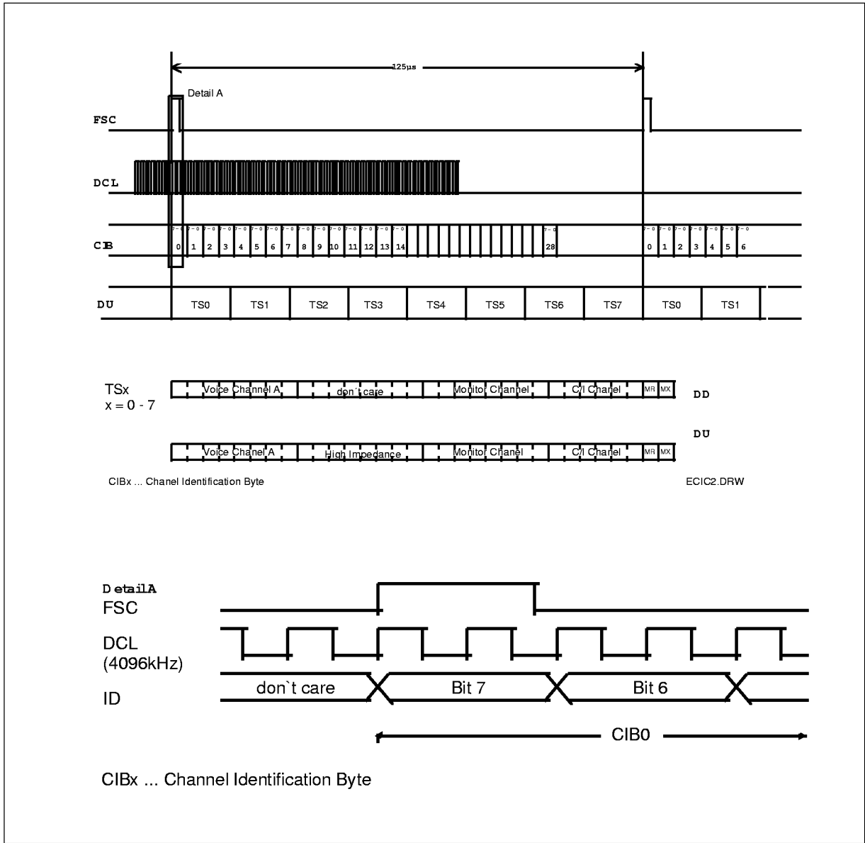
Figure 45 General Timing
