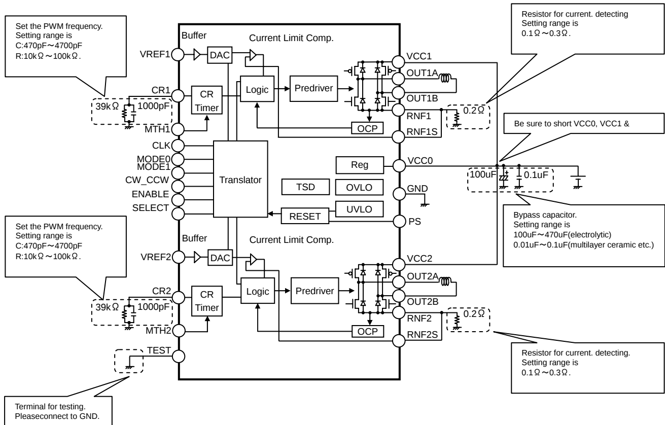
Figure 1. Block diagram &amp; Application circuit diagram of BD6385EFV
