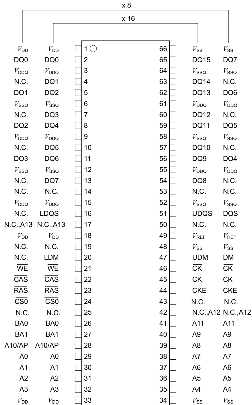
FIGURE 1 Chip Configuration PG-TSOPII-66
