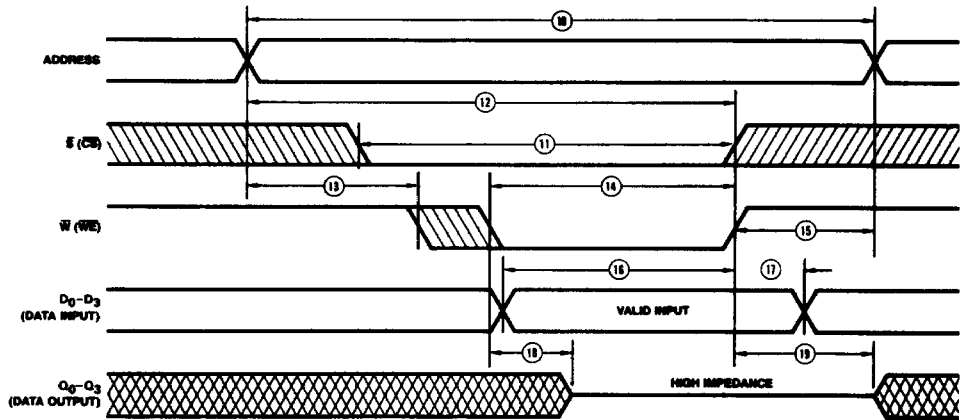
Write Cycle
