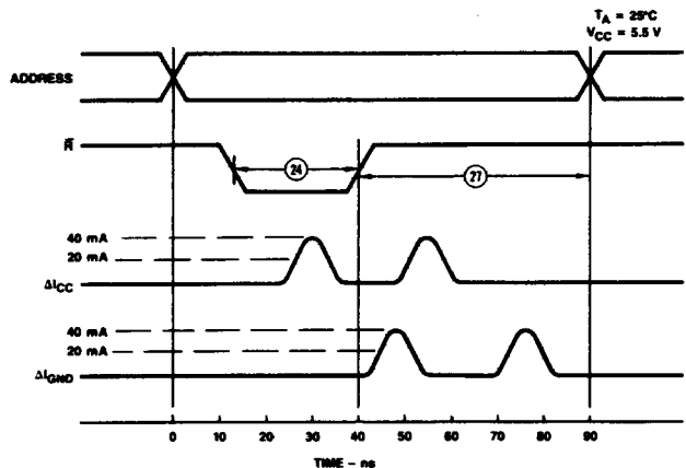
Typical I_{CC} and I_{GND} During a Reset Cycle
