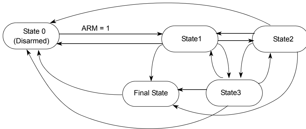
Figure 68. State Sequencer Diagram
