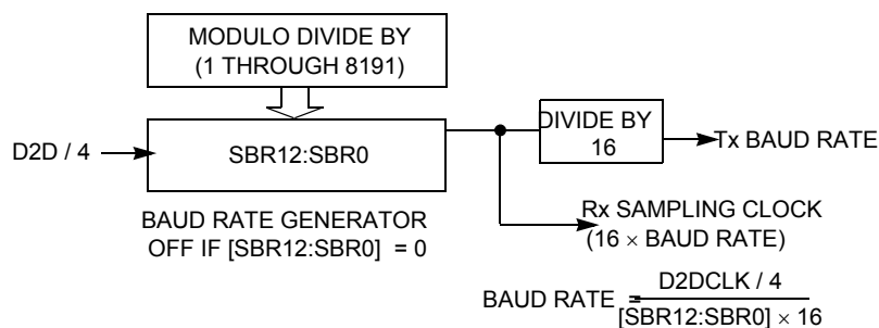
Figure 108. SCI Baud Rate Generation
