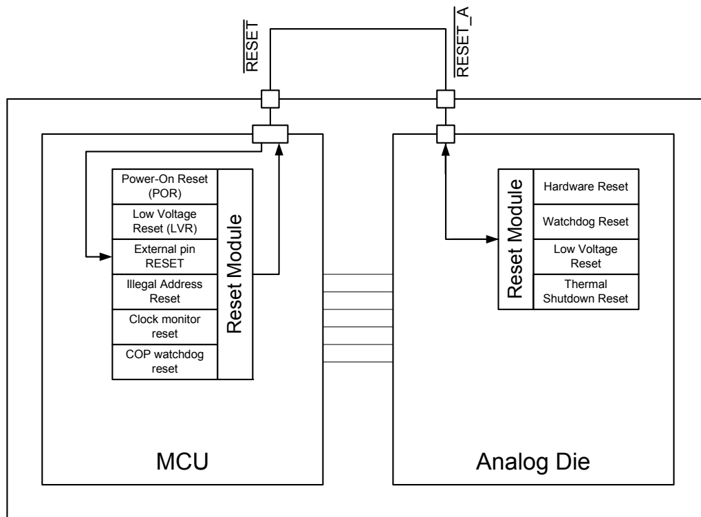
Figure 40. Device Reset Overview
