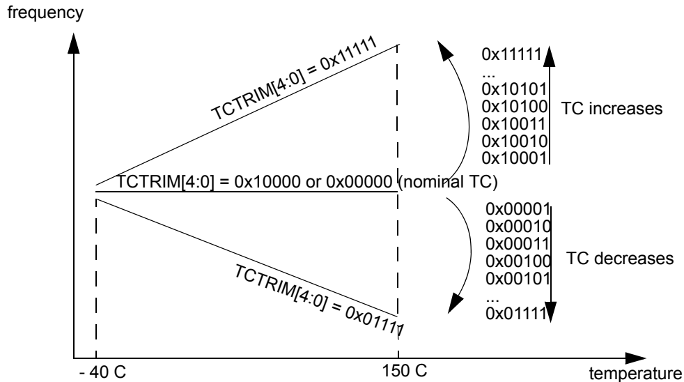
Figure 23. Influence of TCTRIM[4:0] on the Temperature Coefficient
