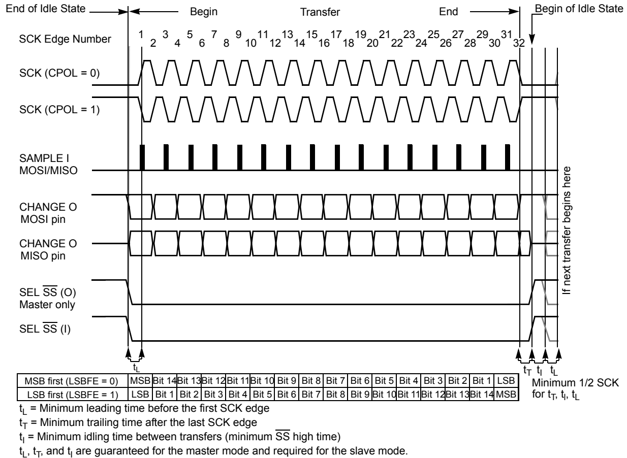
Figure 85. SPI Clock Format 0 (CPHA = 0), with 16-Bit Transfer Width Selected (XFRW = 1)
