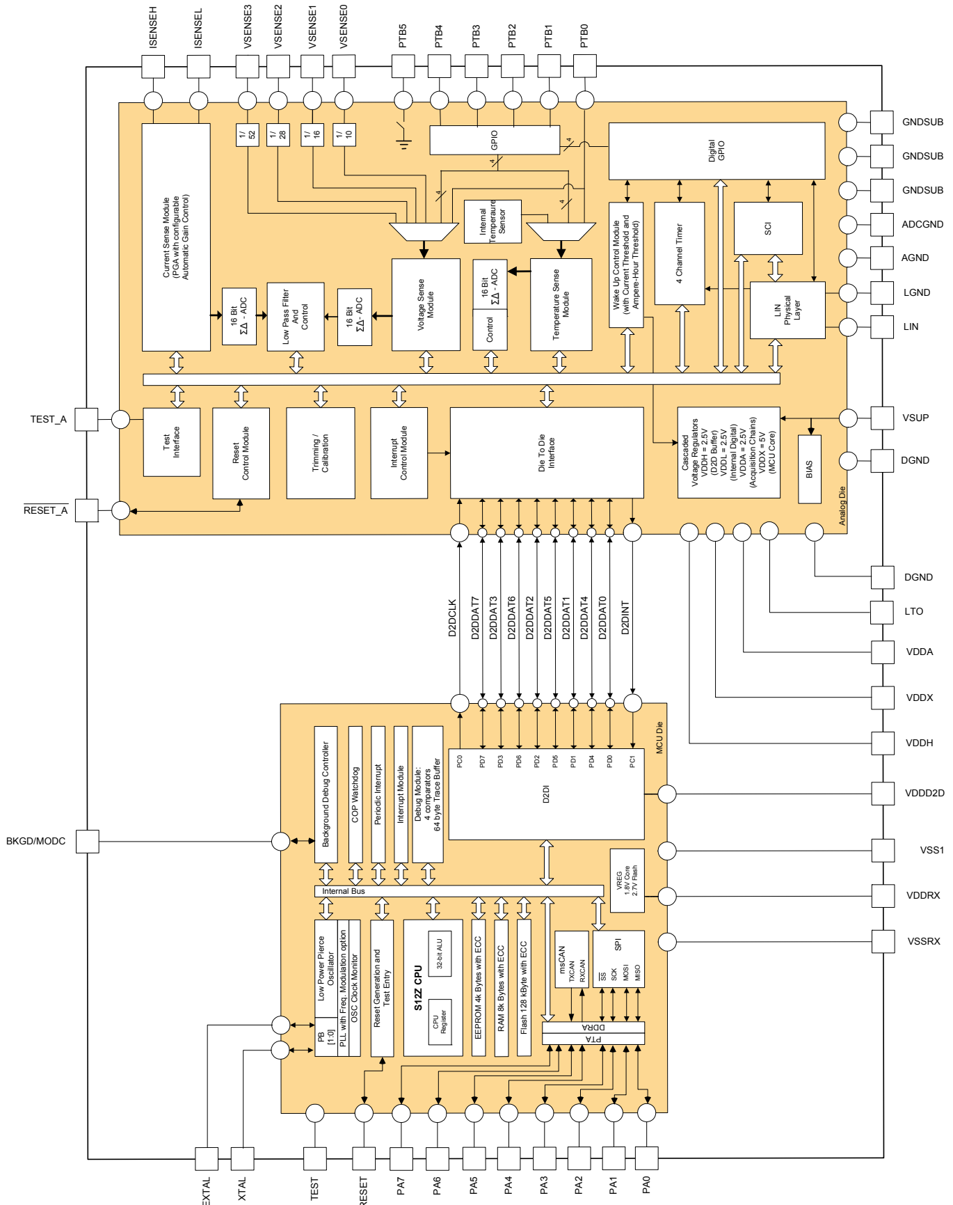
Figure 3. Detailed Block Diagram
