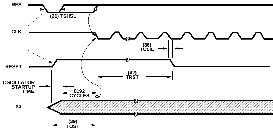
FIGURE 14. RESET TIMING (OSCILLATOR STOPPED, \overline{\text{F/C}} LOW)
