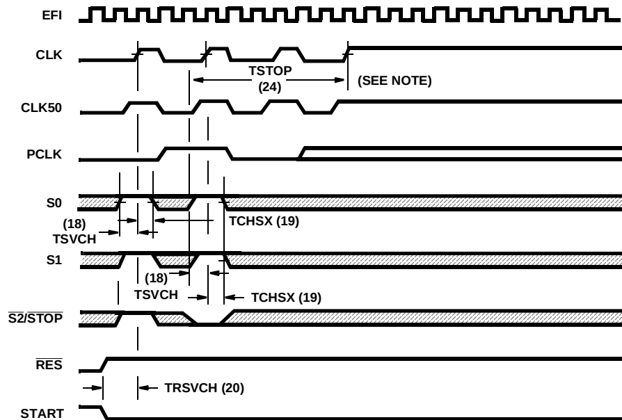
FIGURE 10. CLOCK STOP ( F/\overline{C} HIGH OR F/\overline{C} LOW)
