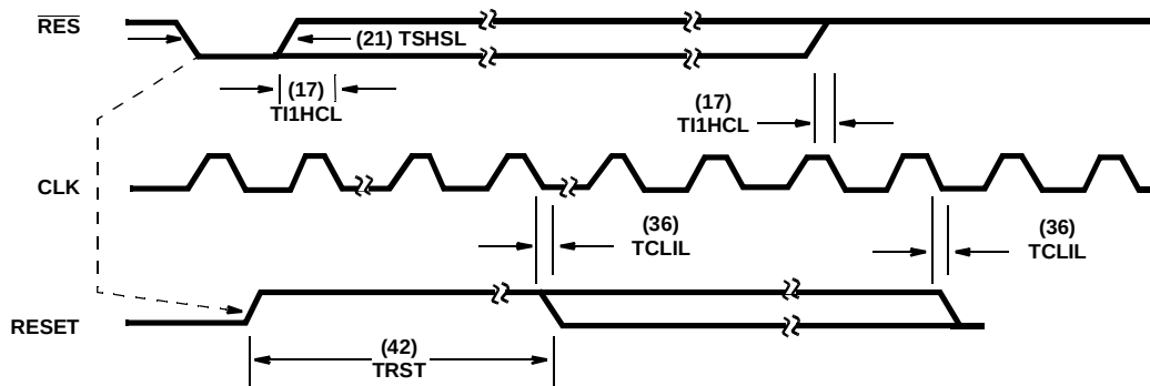
FIGURE 13. RESET TIMING (CLK RUNNING WITH \overline{\text{F/C}} LOW-OSC MODE) (CLK RUNNING-OR STOPPED WITH \overline{\text{F/C}} HIGH EFI MODE)
