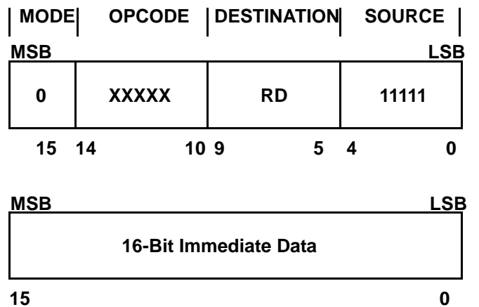
Figure 31c. Register Immediate Instruction Format
