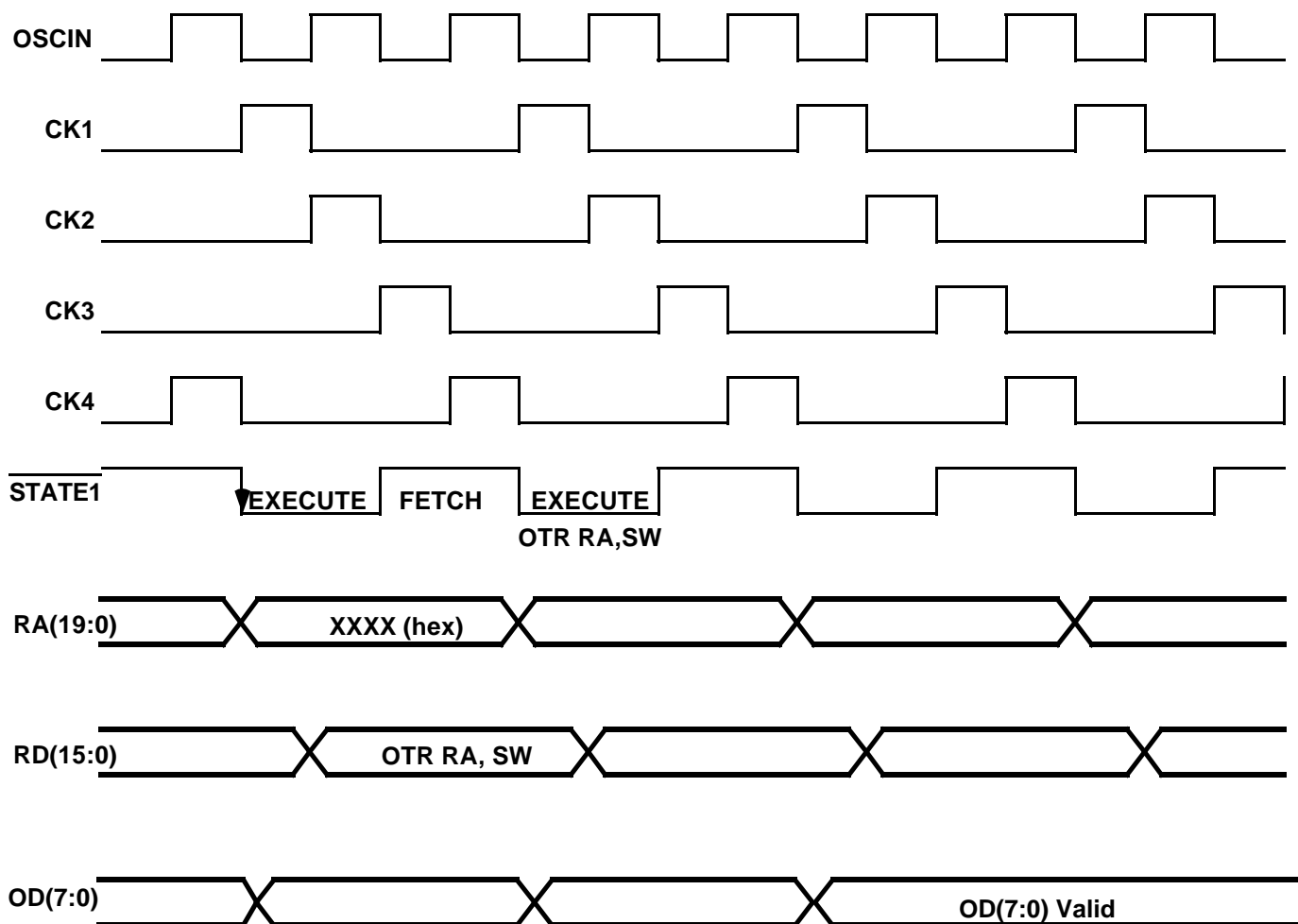
Figure 23. Output Discrete Bus Timing
