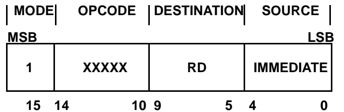
Figure 31b. Register to-Short Immediate Instruction Format
