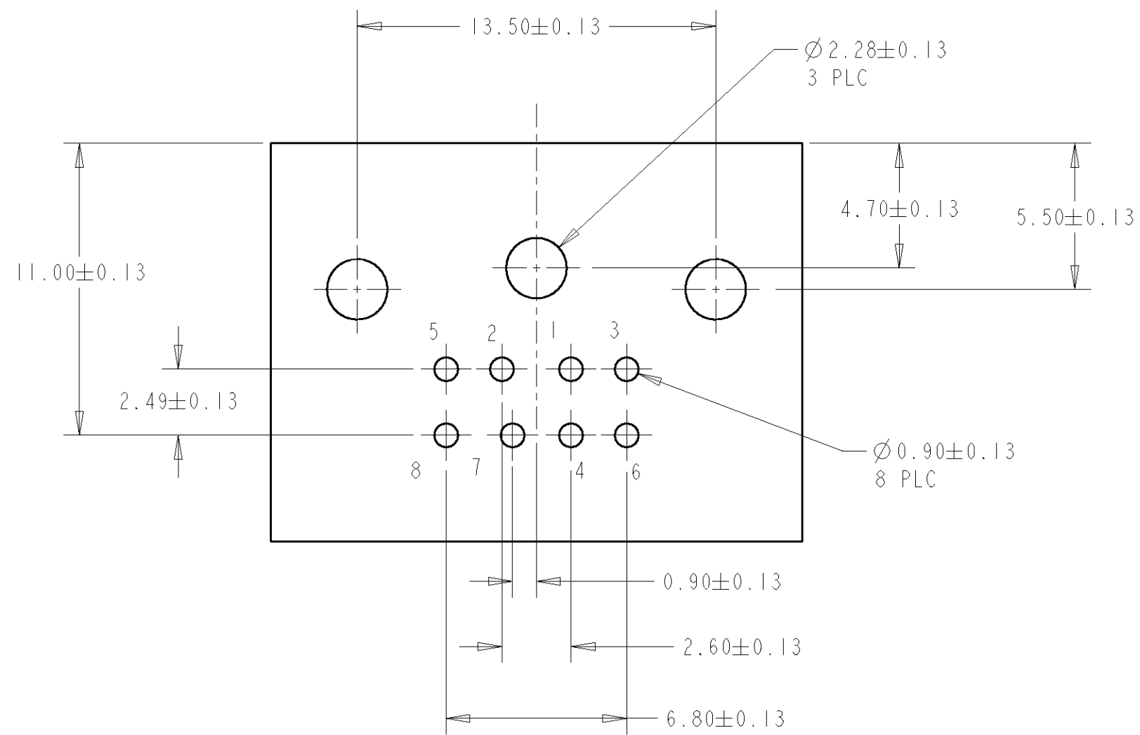
RECOMMENDED PCB LAYOUT BOTTOM VIEW SCALE 5:1
