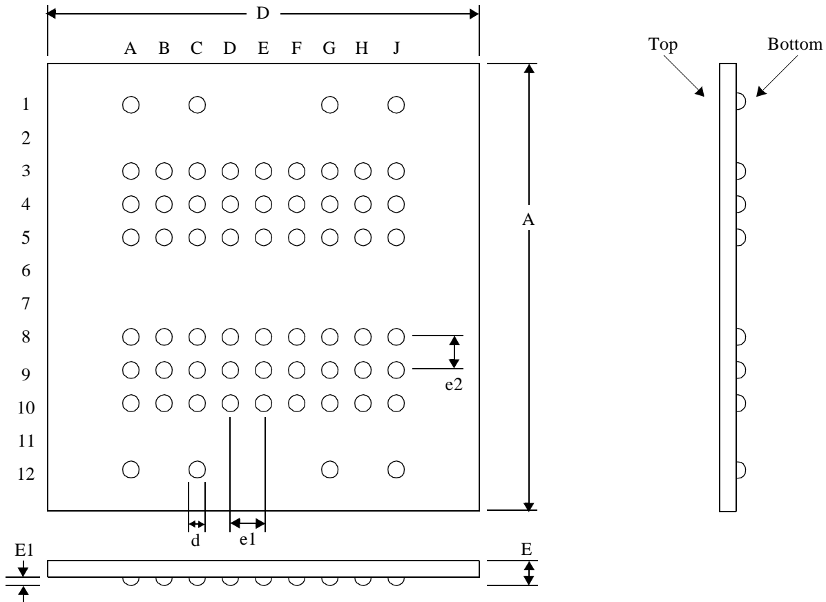
Figure 60: Center-Bonded uBGA Package
