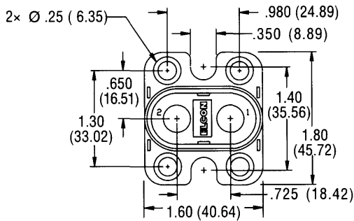
Front Views
