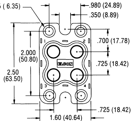
Front Views
