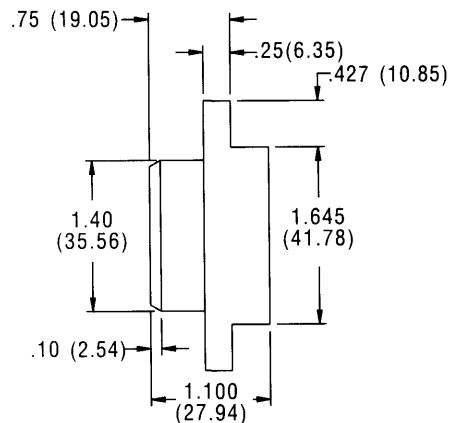
Socket side
