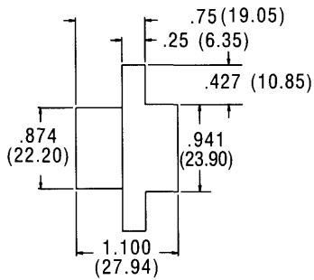
Pin side
