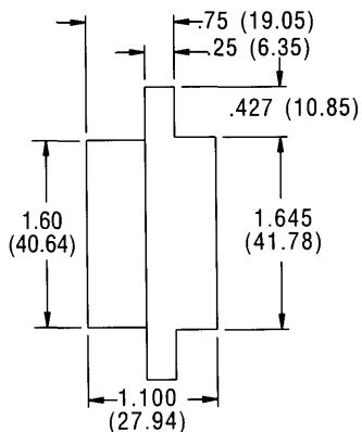
Pin side
