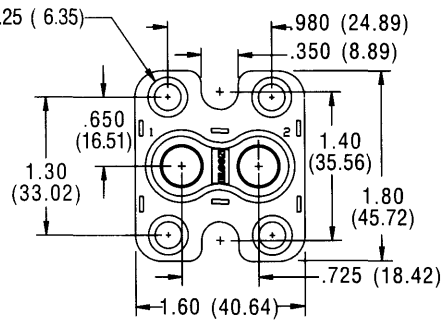
Front Views
