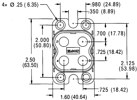
Front Views
