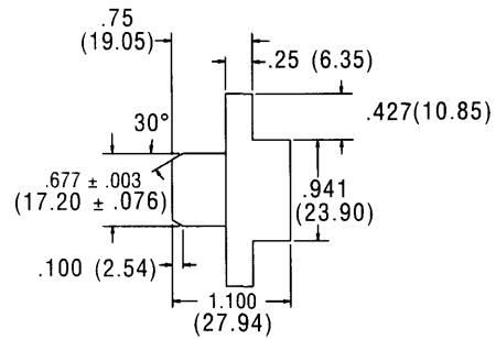
Socket side
