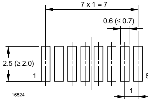
Figure 7. TFDU5102 Baby Face (Universal)
