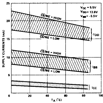
RANGE OF SUPPLY CURRENTS VS. TEMPERATURE
