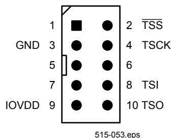
Figure 6-1 ISD/ISP Connector
