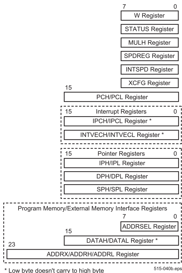
Figure 3-3 CPU Registers
