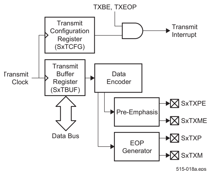
Figure 5-11 Transmit Data Paths
