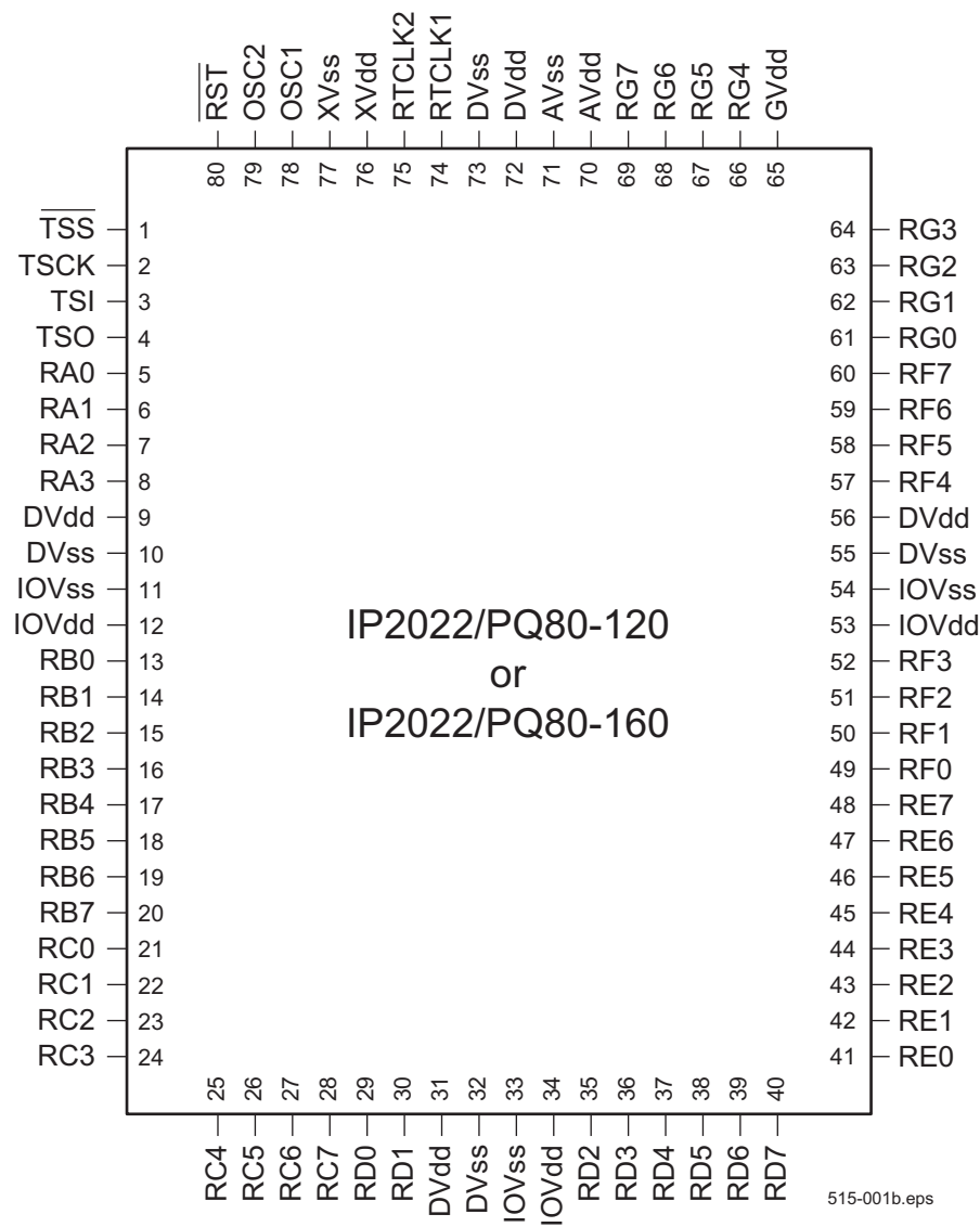
Figure 2-1 IP2022 PQFP Pin Definition (Top View)
