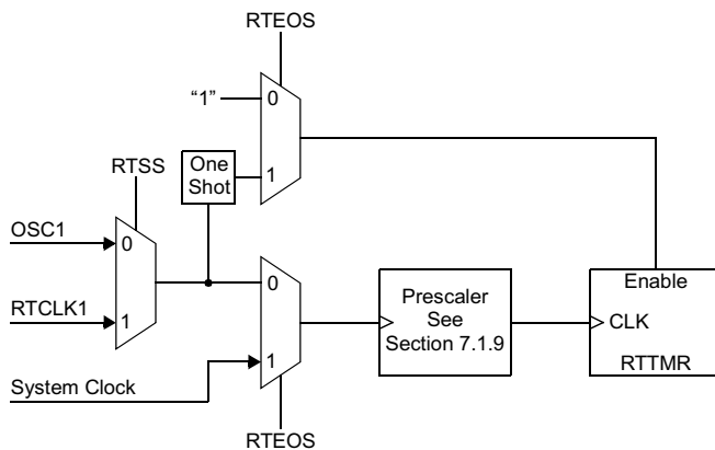
Figure 5-4 Real-Time Timer Block Diagram
