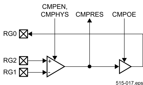
Figure 5-18 Analog Comparator
