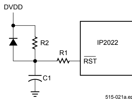
Figure 3-16 External Reset Circuit
