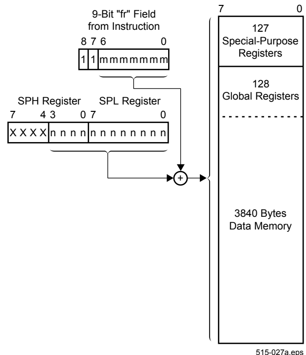
Figure 4-5 Indirect-with-Offset Mode, Stack Pointer
