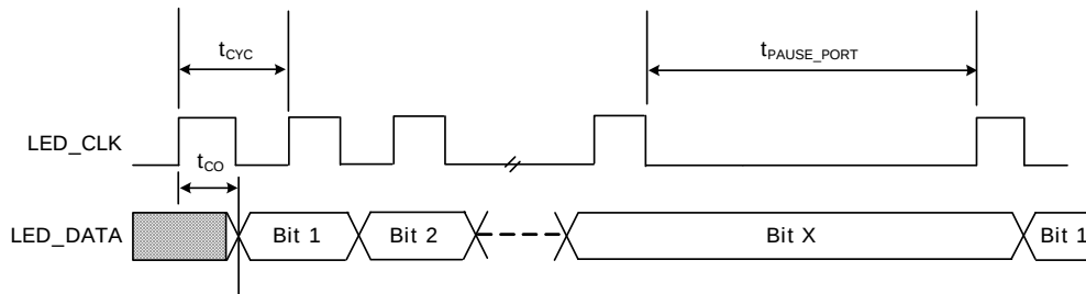
Figure 24 • Basic Serial LED Timing
