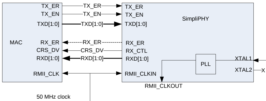
Figure 6 • Mode 1
