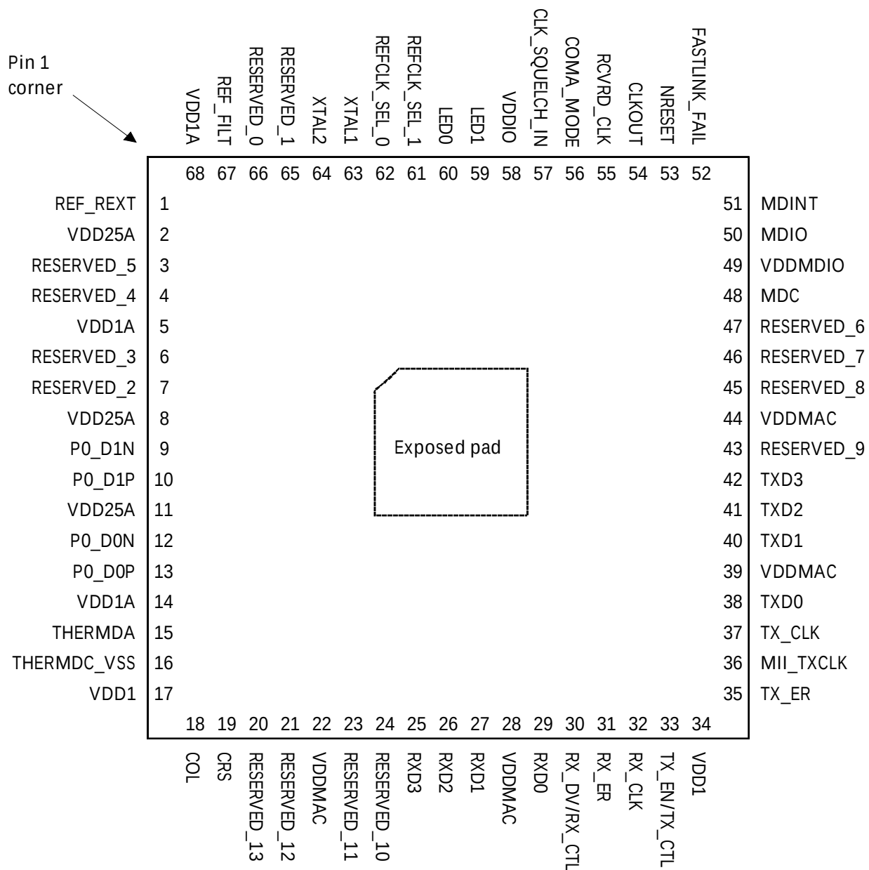
Figure 31 • Pin Diagram
