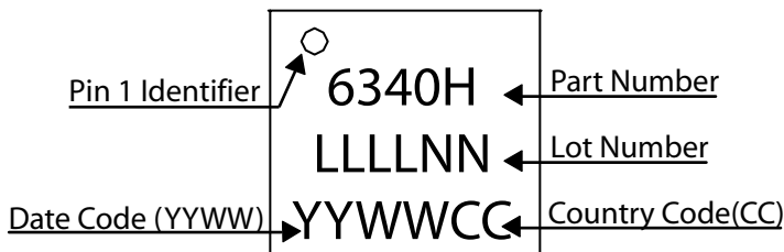
Figure 6: Branding Specification - M45 Package
