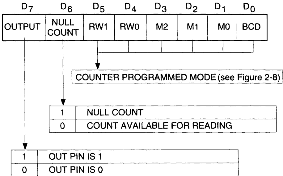
Figure 2-11: Status Byte
