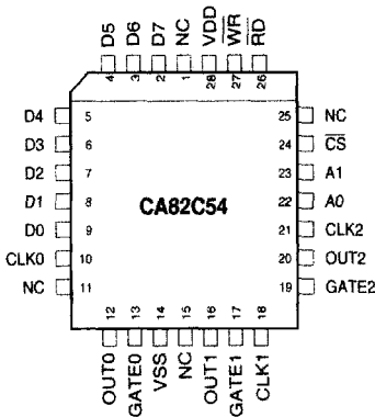
Figure 2-1: PLCC Pin Configurations
