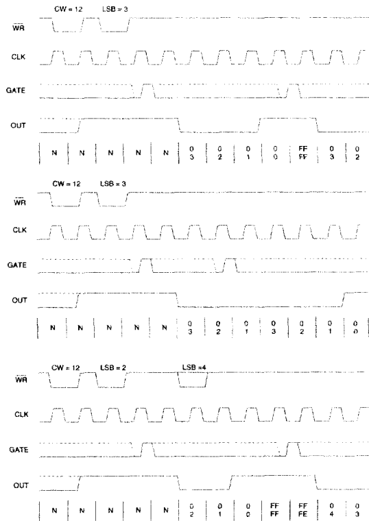
Figure 2-13: Mode 1 Timing
