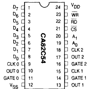
Figure 2-2: PDIP Pin Configurations
