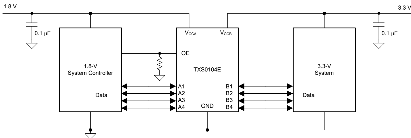
Figure 9-1. Application Schematic
