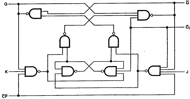
LOGIC DIAGRAMS (one half shown) '73, 'H73
