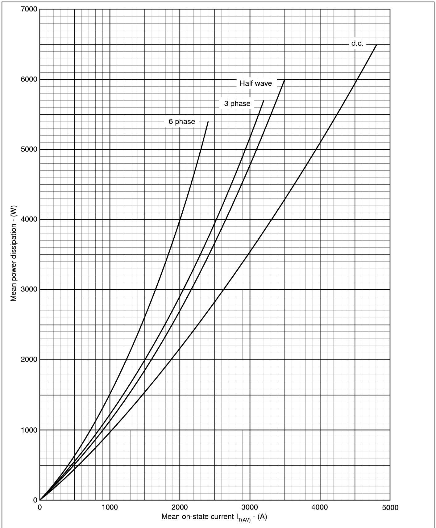
Fig.2 Dissipation curves
