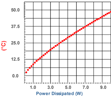
Heat Sink Temperature Rise Above Ambient
