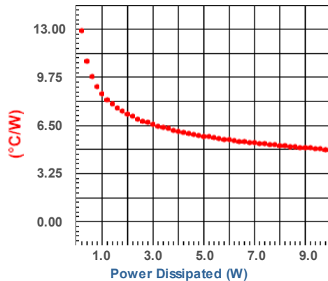
Heat Sink Thermal Resistance
