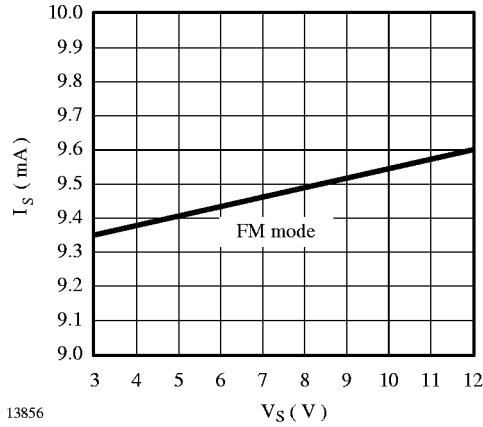
Figure 40. Supply-current characteristic
