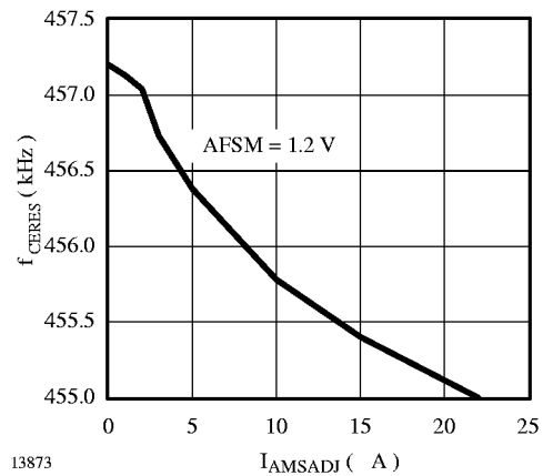
Figure 14. Pulling characteristic
