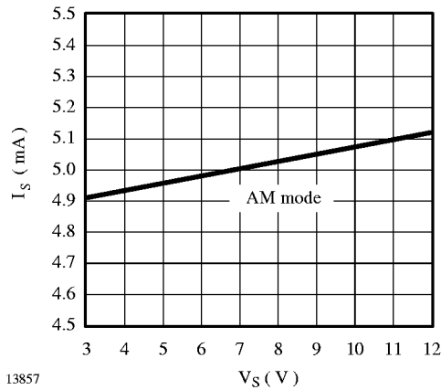
Figure 41. Supply-current characteristic
