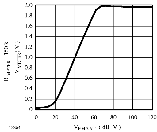
Figure 51. FM field-strength characteristic
