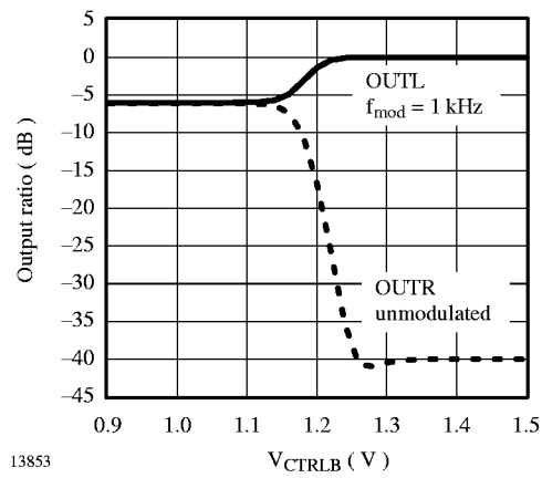
Figure 33. Forced mono function
