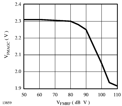
Figure 6. FM AGC characteristic
