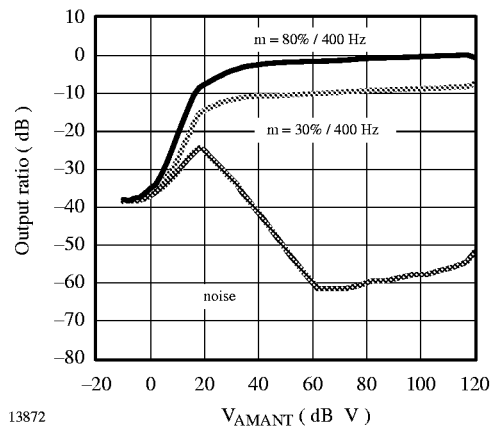
Figure 53. AM signal and noise characteristic
