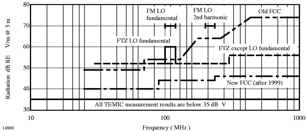
Figure 62. FCC measurements
