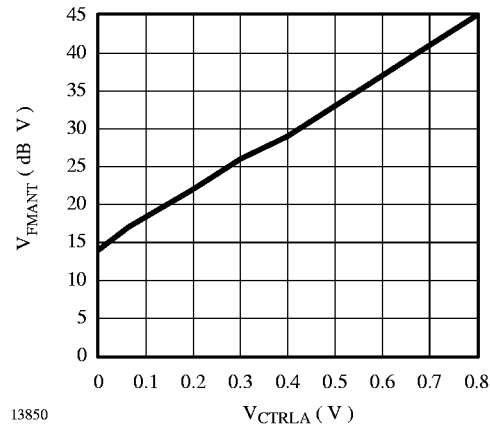
Figure 29. Adjustable FM stop-signal sensitivity
