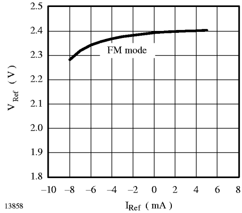
Figure 43. Load characteristic of V_{Ref}
