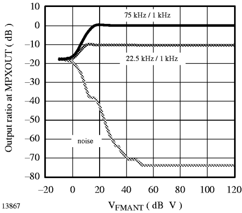
Figure 46. FM signal and noise characteristic
