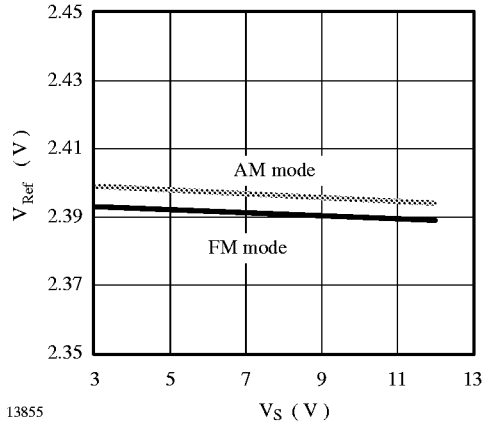
Figure 39. Supply-voltage characteristic of V_{Ref}
