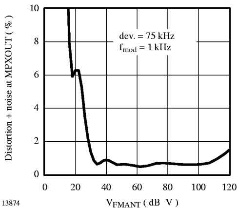
Figure 47. FM distortion and noise characteristic at MPXOUT
