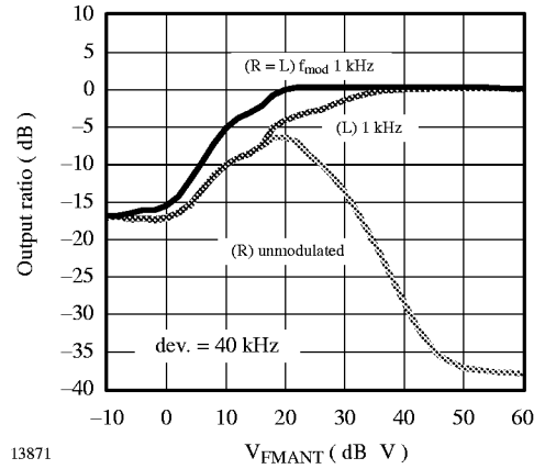
Figure 49. Channel-separation characteristic
