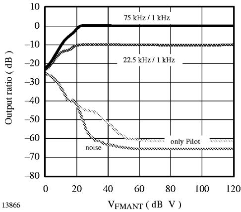
Figure 45. FM signal and noise characteristic
