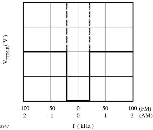
Figure 38. Stop signal
