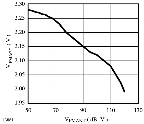
Figure 4. FM AGC characteristic
