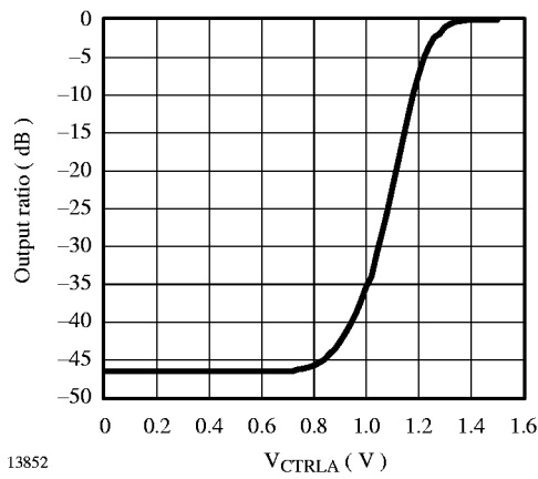
Figure 31. Mute function
