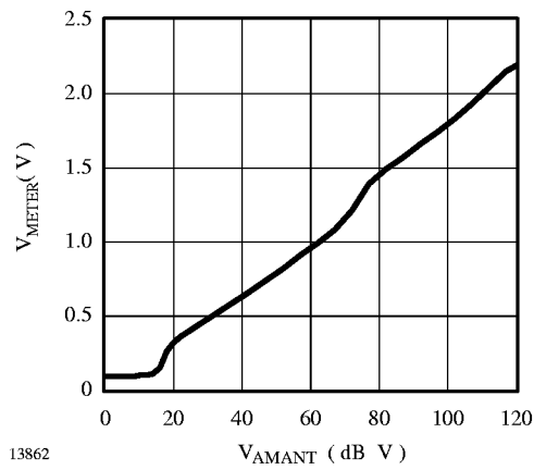
Figure 52. AM field-strength characteristic
