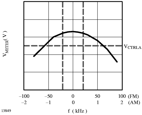
Figure 36. Field-strength tuning characteristic
