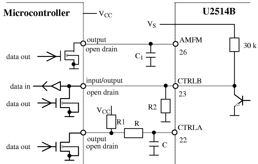
I/O Ports of microcontroller
