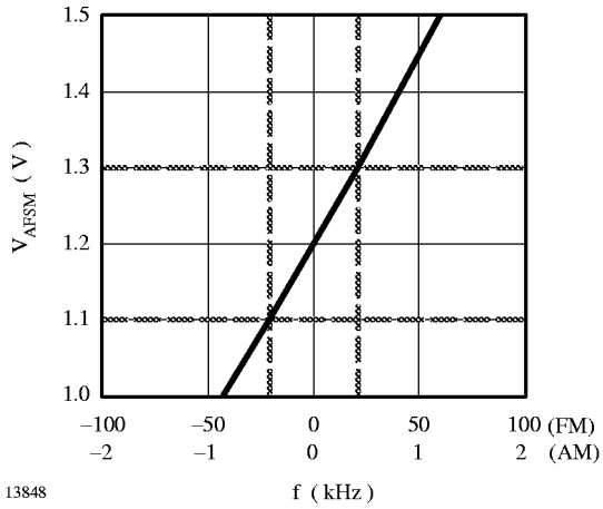
Figure 37. Smoothed S-curve
