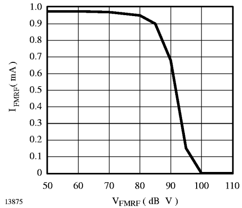
Figure 5. FM AGC characteristic
