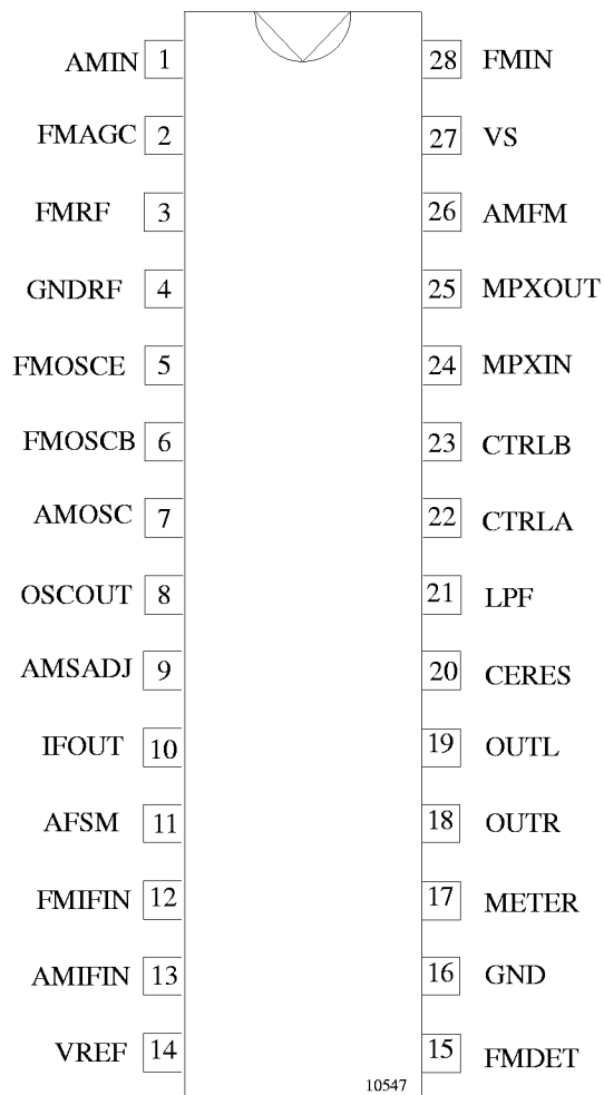
Figure 2. Pinning
