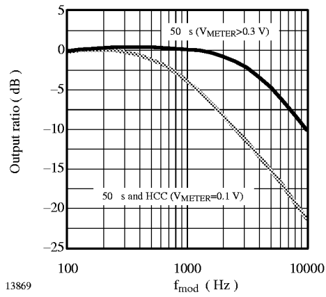
Figure 44. High-cut control (HCC)
