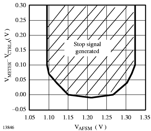
Figure 35. Stop signal in AM search mode
