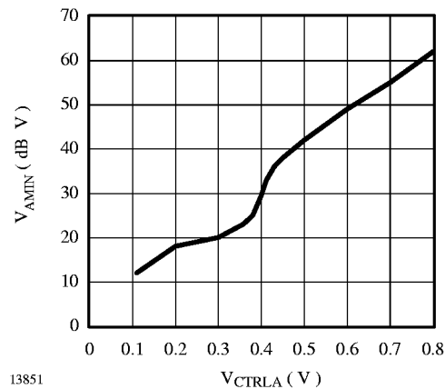
Figure 30. Adjustable AM stop-signal sensitivity
