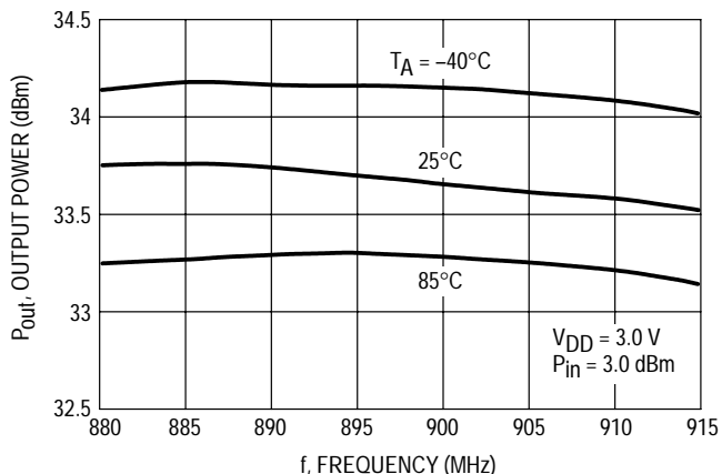
Figure 6. Output Power versus Frequency
