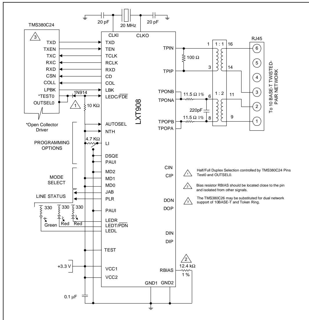
Figure 10. Full-Duplex Operation
