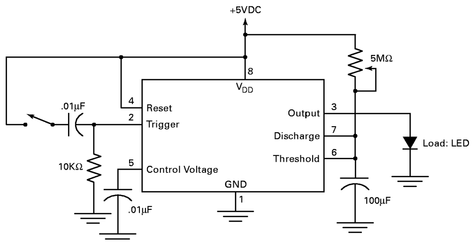
FIGURE 8. AN INDUSTRY-STANDARD 555 NONRETRIGGERABLE APPLICATION
