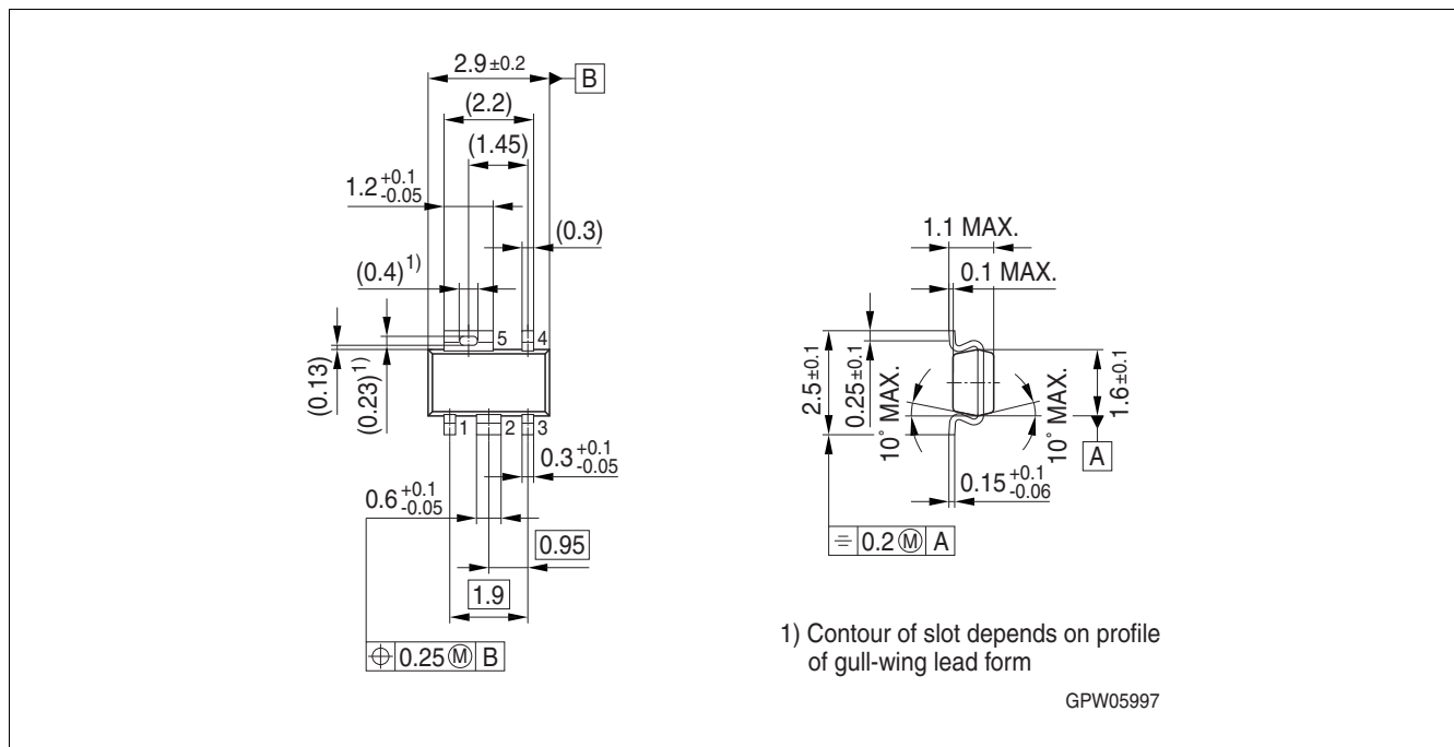
Figure 4 PG-SCT595-5¹)
