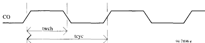
Figure 16. Clock output (CO)
