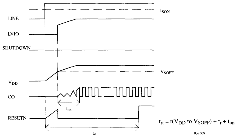
Figure 12. Power on in speed-up condition ( V_{DD} < V_{SON} )
