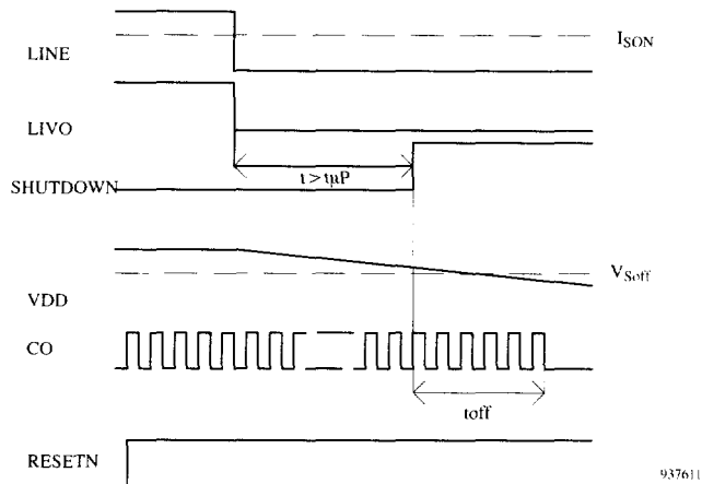
Figure 14. Line break
