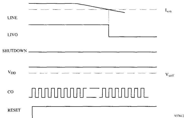
Figure 15. Line current fall
