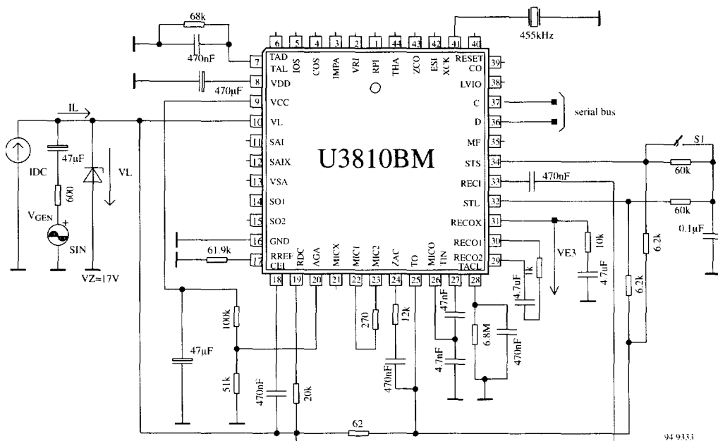
Figure 7. Test circuit for receive
