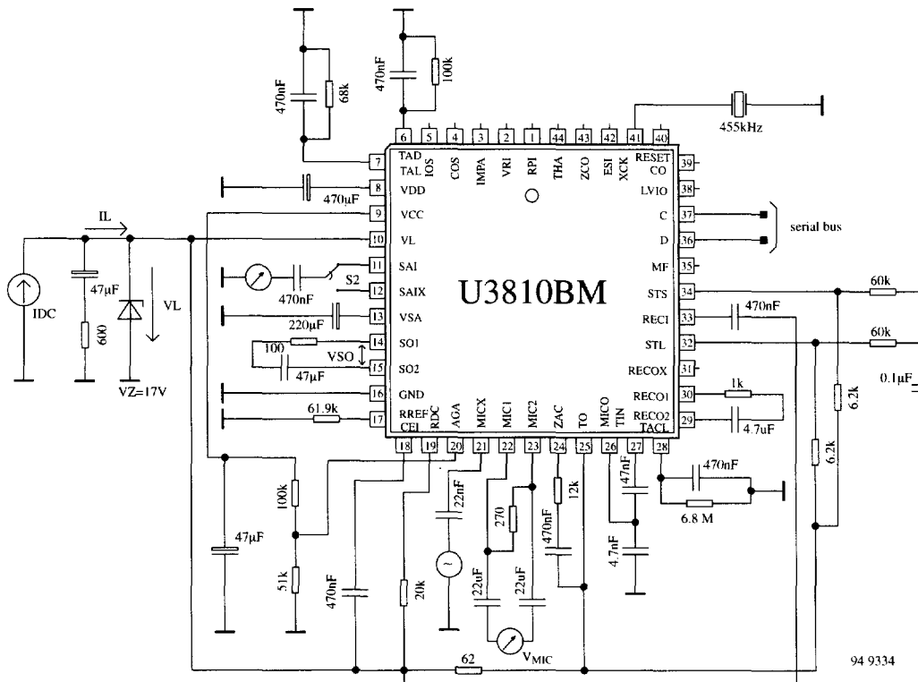
Figure 8. Test circuit for speaker amplifier
