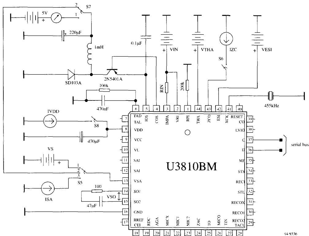
Figure 10. Test circuit for ringer
