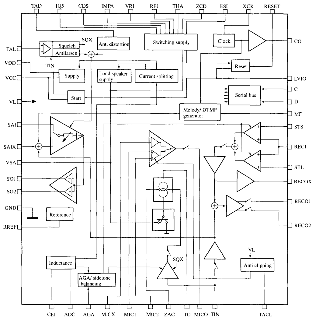
Figure 2. Detailed block diagram
