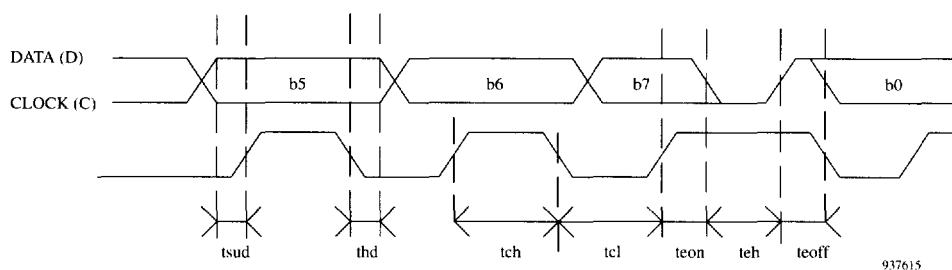
Figure 20. Serial bus timing
