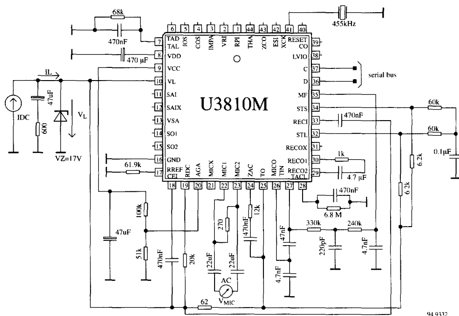
Figure 6. Test circuit for transmission
