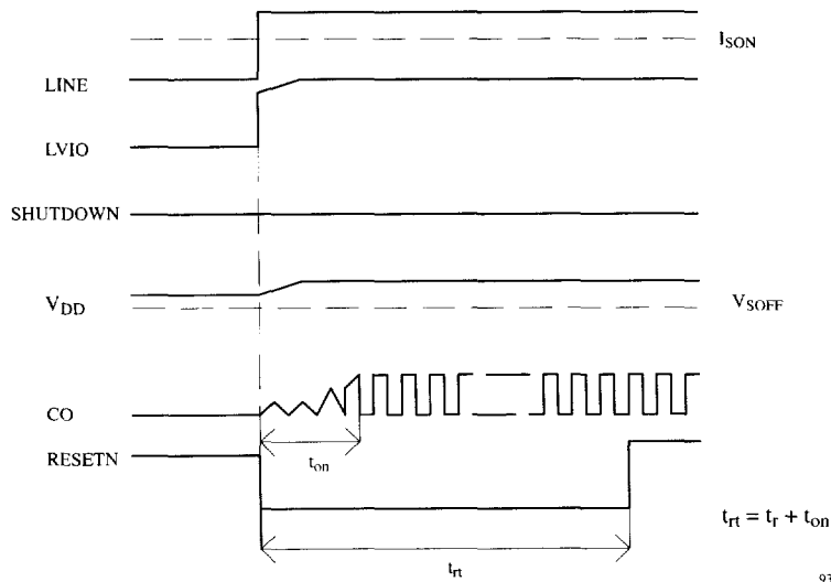
Figure 13. Power on without speed-up ( V_{DD} > V_{SON} )
