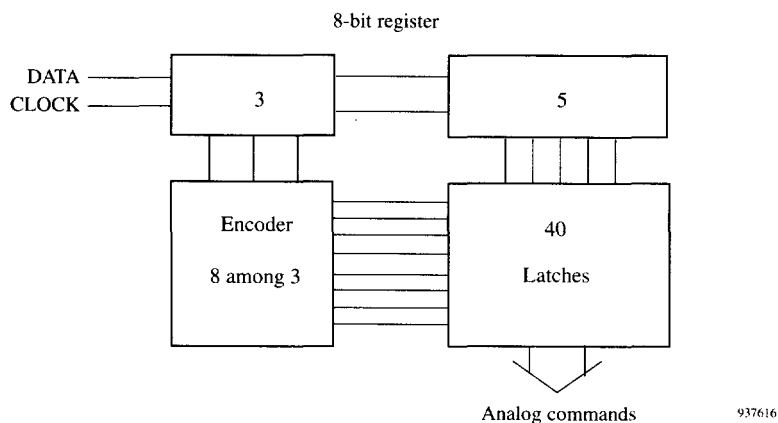
Figure 19. Serial bus interface
