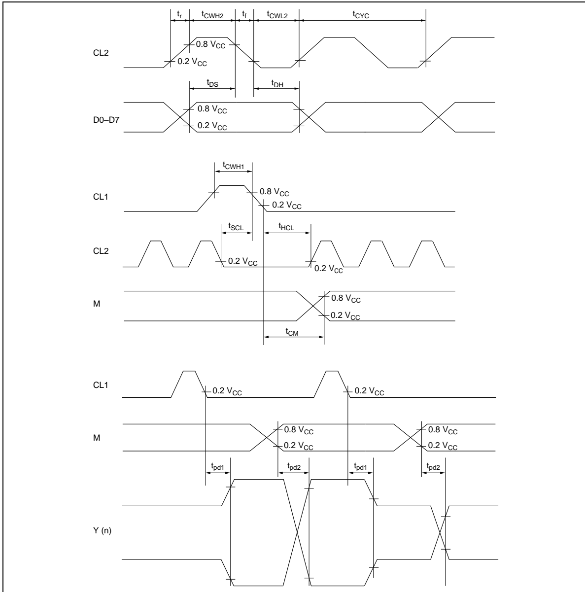
Figure 8 LCD Controller Interface Timing
