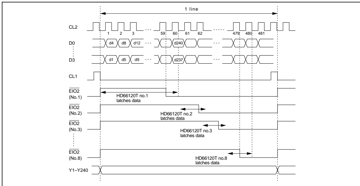
Figure 4 4-Bit Data Latch Timing (BS = GND, 1 Line: 640-by-3 Dots)
