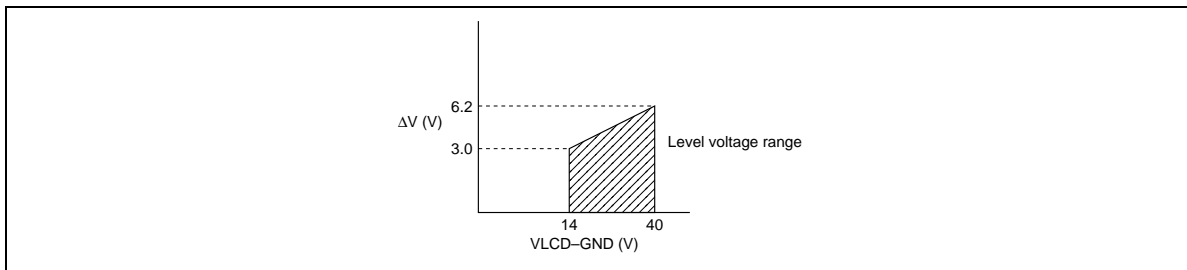
Figure 7 Relation between VLCD-GND and \Delta V
