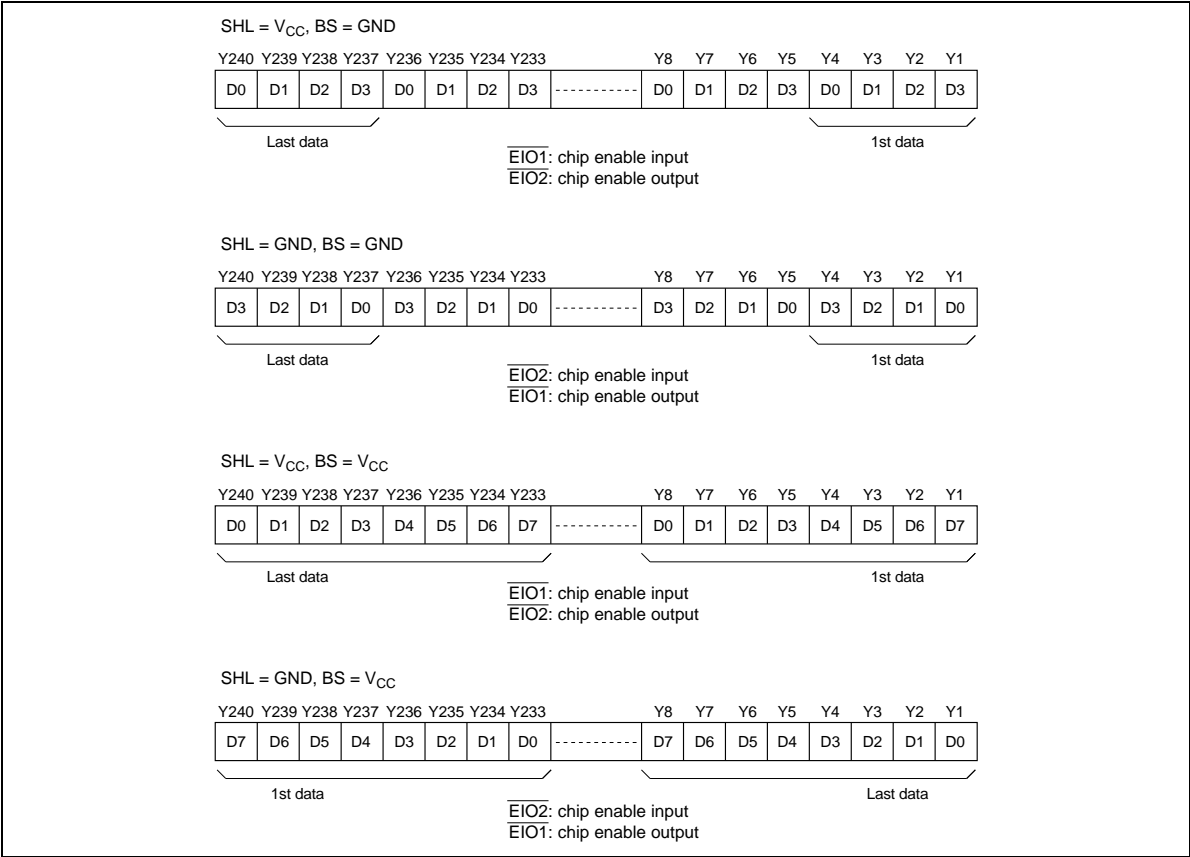
Figure 2 Selection of Destinations of Display Data Output
