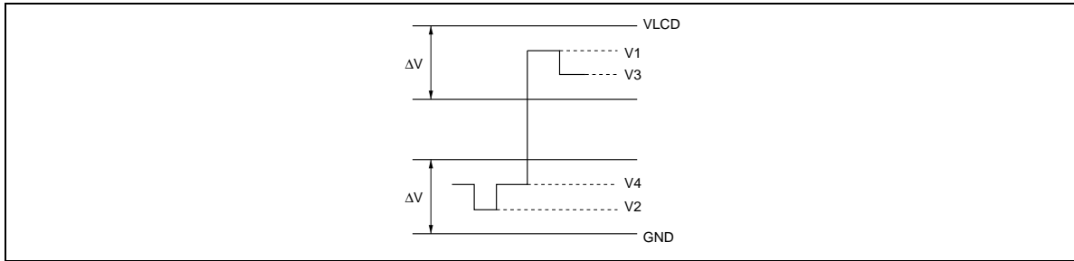
Figure 6 Relation between Driver Output Waveform and Level Voltages
