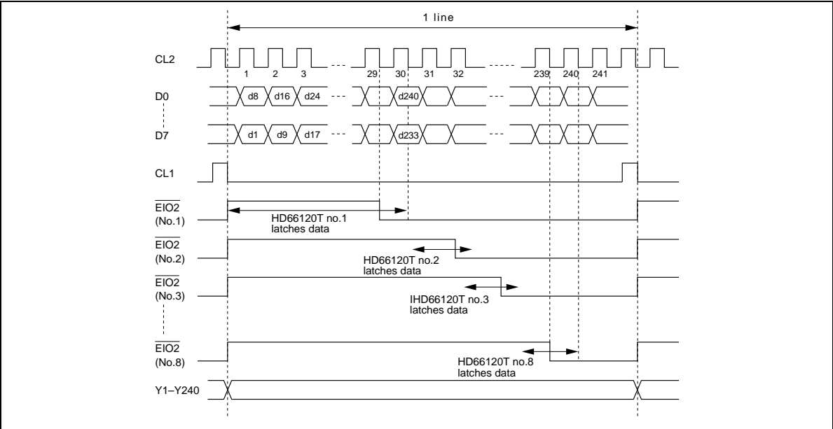
Figure 5 8-Bit Data Latch Timing (BS = V cc , 1 Line: 640-by-3 Dots)
