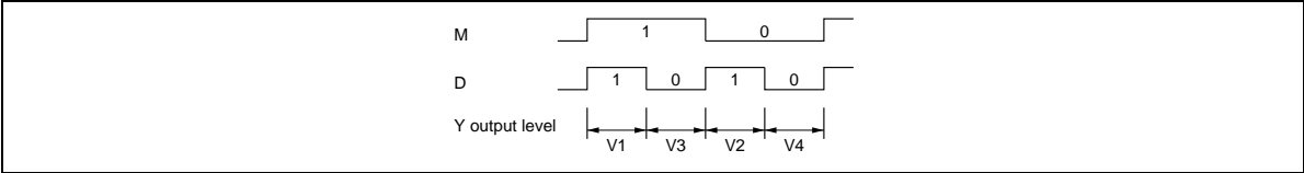
Figure 3 Selection of LCD Drive Output Level
