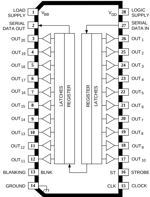
A6812xLW (SOIC)
