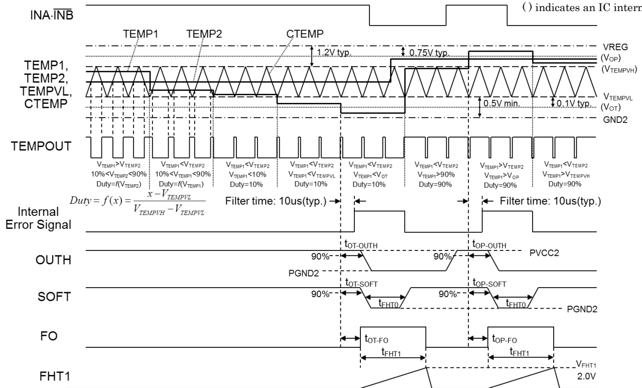
Figure 20: IGBT Temperature Monitor
