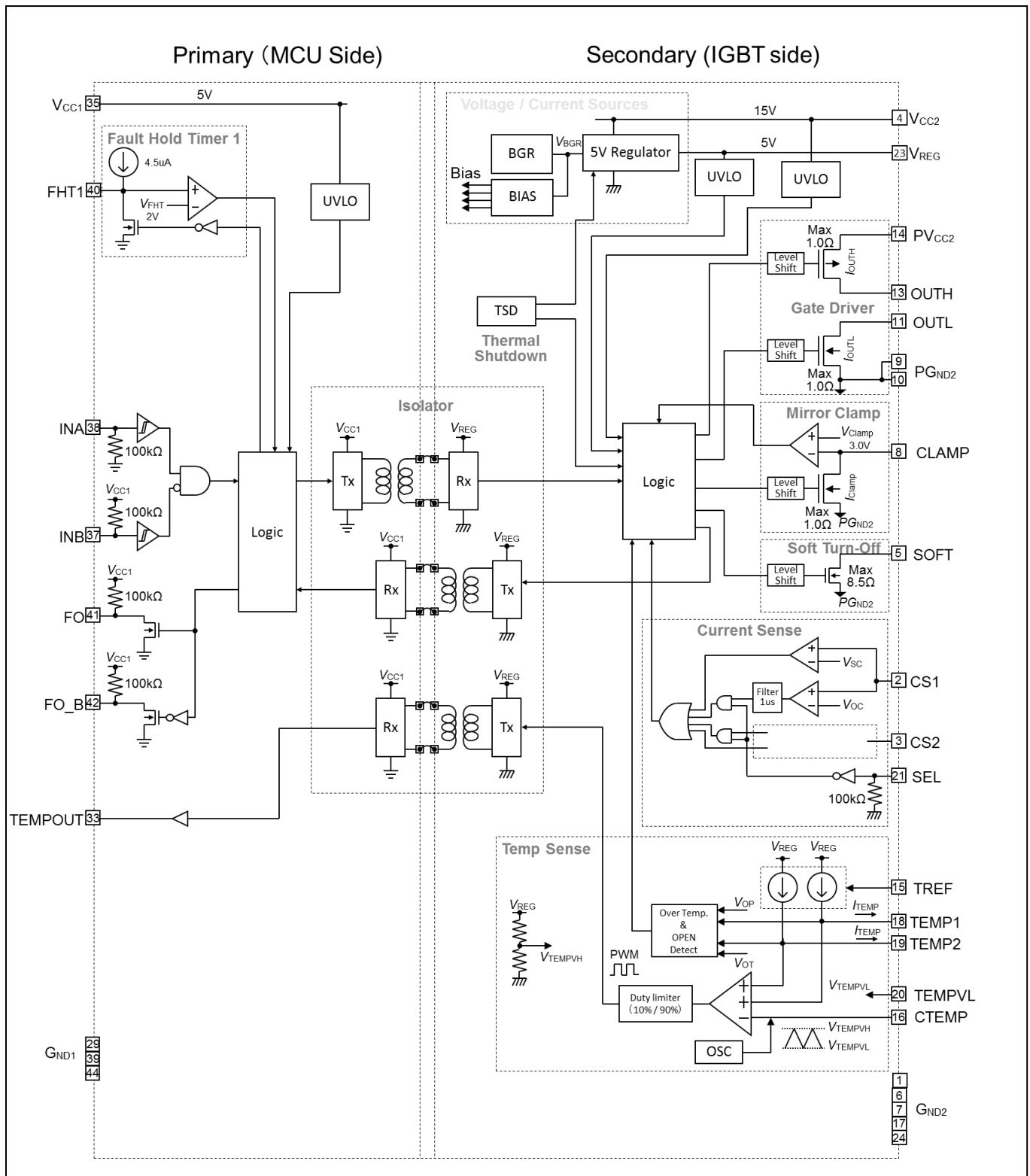
Figure 1: Block Diagram
