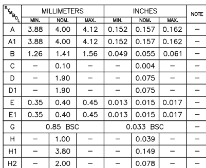
Figure 4: M7 Package Outline - 10 Pin 4 mm x 4 mm x 1.5 mm Surface Mount Module
