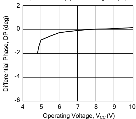
Differential Phase vs. Operating Voltage ( T_a = 25^\circ\text{C} , 1Vp-p staircase signal input)
