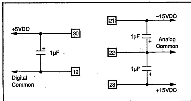
FIGURE 8. Recommended Power Supply Decoupling.
