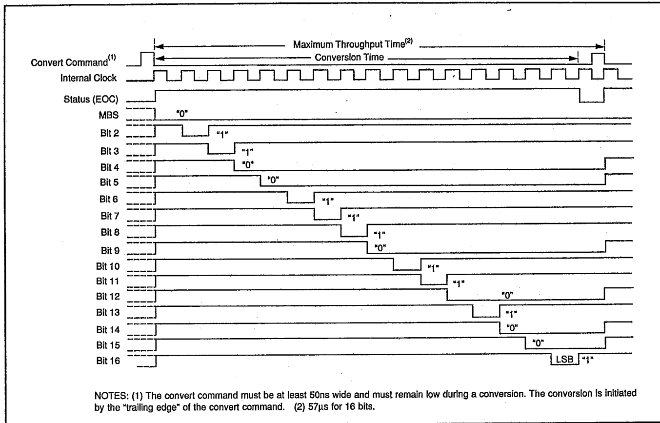
FIGURE 2. ADC71 Timing Diagram.
