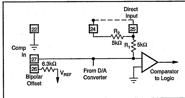
FIGURE 9. ADC71 Input Scaling Circuit.
