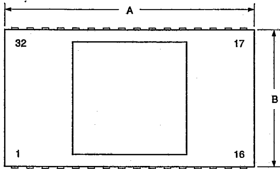
H Package — 32-Pin Hermetic DIP
