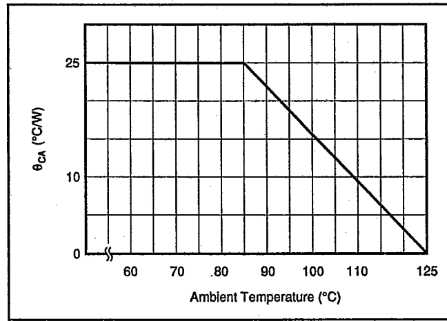
FIGURE 10. \theta_{CA} Requirement Above 85°C.
