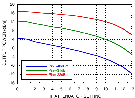
Figure 9. 60.48 GHz (IEEE CH-2) Output Power vs. IF Gain Setting [3][4]
