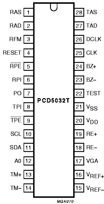
Fig.3 Pin configuration SO28 (SOT136-1).
